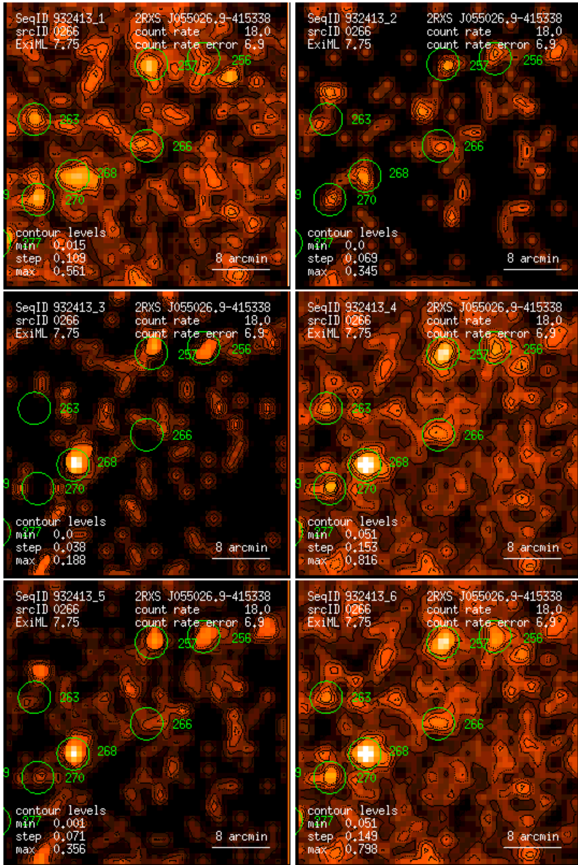
Figure 266: RASS 932413: detection 0266: band rate images, Gaussian filter: (1) PSPC channels 11 – 41, (2) 52 – 90, (3) 91 – 201, (4) 11 – 235, (5) 52 – 201, (6) 11 – 201. Broad band rates in counts/ks. Band rate contour levels in counts/ks/arcmin 2 .
