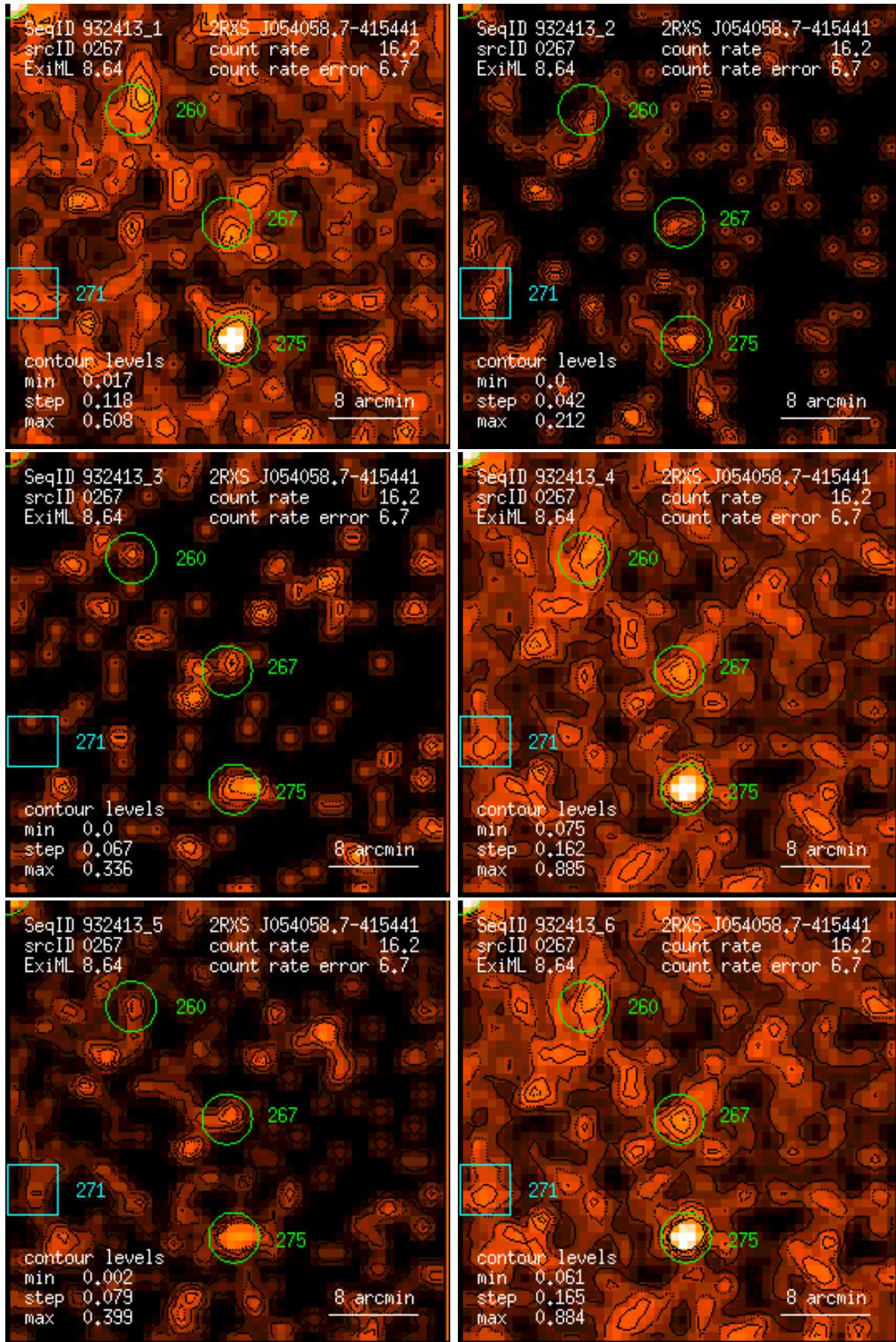
Figure 267: RASS 932413: detection 0267: band rate images, Gaussian filter: (1) PSPC channels 11 – 41, (2) 52 – 90, (3) 91 – 201, (4) 11 – 235, (5) 52 – 201, (6) 11 – 201. Broad band rates in counts/ks. Band rate contour levels in counts/ks/arcmin 2 .
