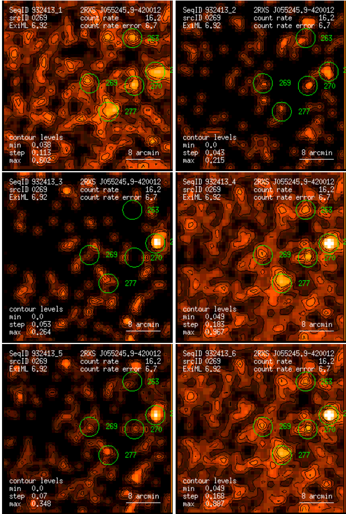
Figure 269: RASS 932413: detection 0269: band rate images, Gaussian filter: (1) PSPC channels 11 – 41, (2) 52 – 90, (3) 91 – 201, (4) 11 – 235, (5) 52 – 201, (6) 11 – 201. Broad band rates in counts/ks. Band rate contour levels in counts/ks/arcmin 2 .
