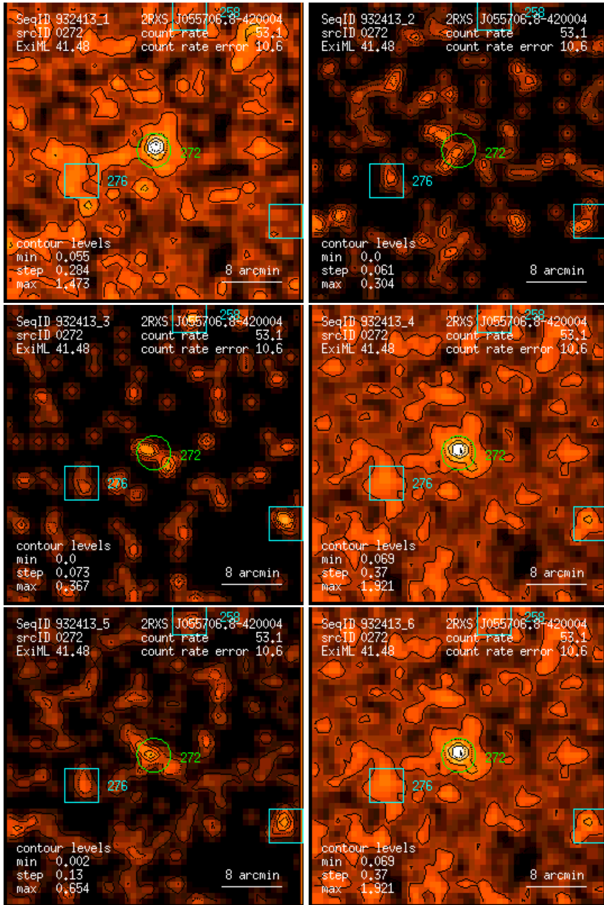
Figure 272: RASS 932413: detection 0272: band rate images, Gaussian filter: (1) PSPC channels 11 – 41, (2) 52 – 90, (3) 91 – 201, (4) 11 – 235, (5) 52 – 201, (6) 11 – 201. Broad band rates in counts/ks. Band rate contour levels in counts/ks/arcmin 2 .
