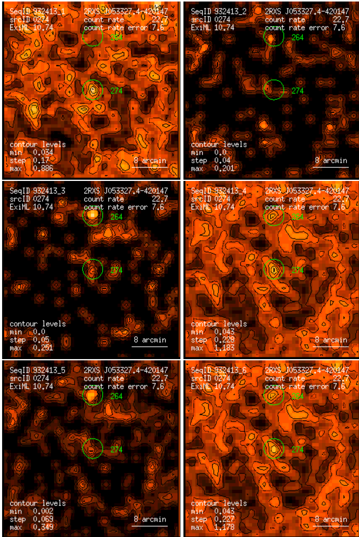
Figure 274: RASS 932413: detection 0274: band rate images, Gaussian filter: (1) PSPC channels 11 – 41, (2) 52 – 90, (3) 91 – 201, (4) 11 – 235, (5) 52 – 201, (6) 11 – 201. Broad band rates in counts/ks. Band rate contour levels in counts/ks/arcmin 2 .
