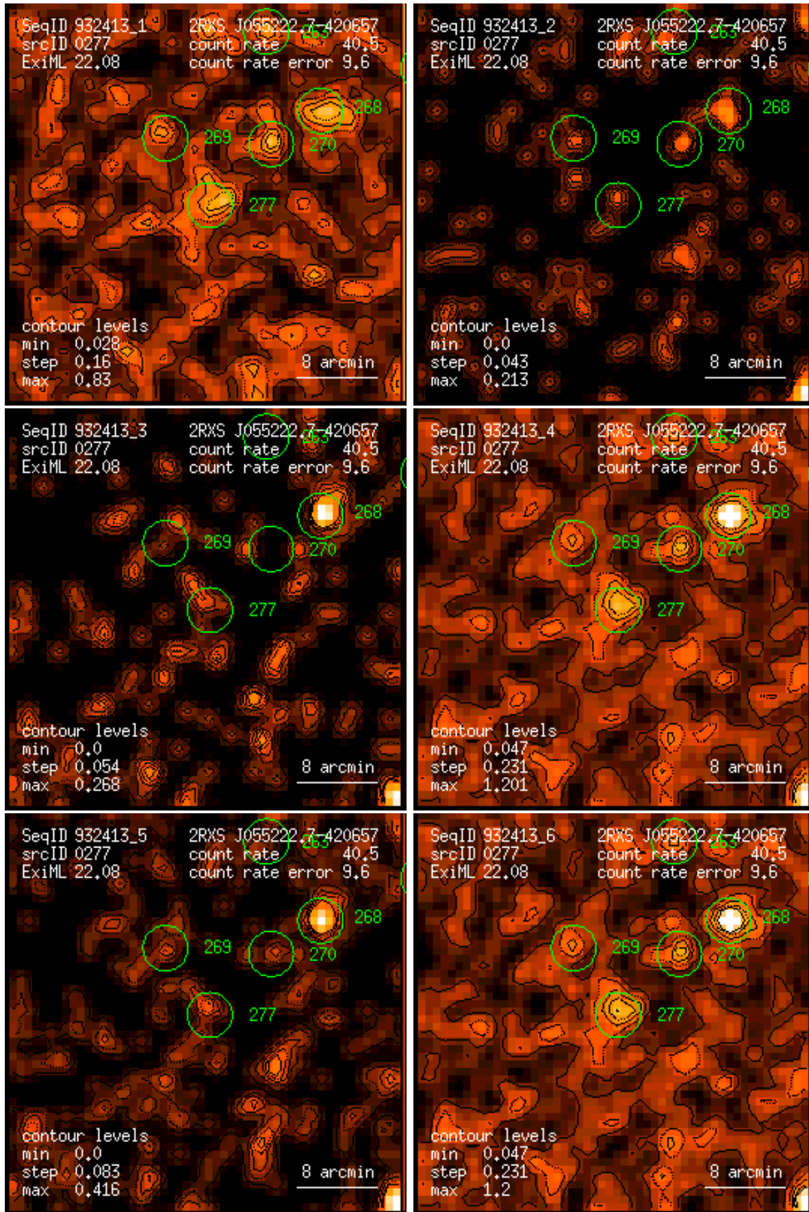
Figure 277: RASS 932413: detection 0277: band rate images, Gaussian filter: (1) PSPC channels 11 – 41, (2) 52 – 90, (3) 91 – 201, (4) 11 – 235, (5) 52 – 201, (6) 11 – 201. Broad band rates in counts/ks. Band rate contour levels in counts/ks/arcmin 2 .
