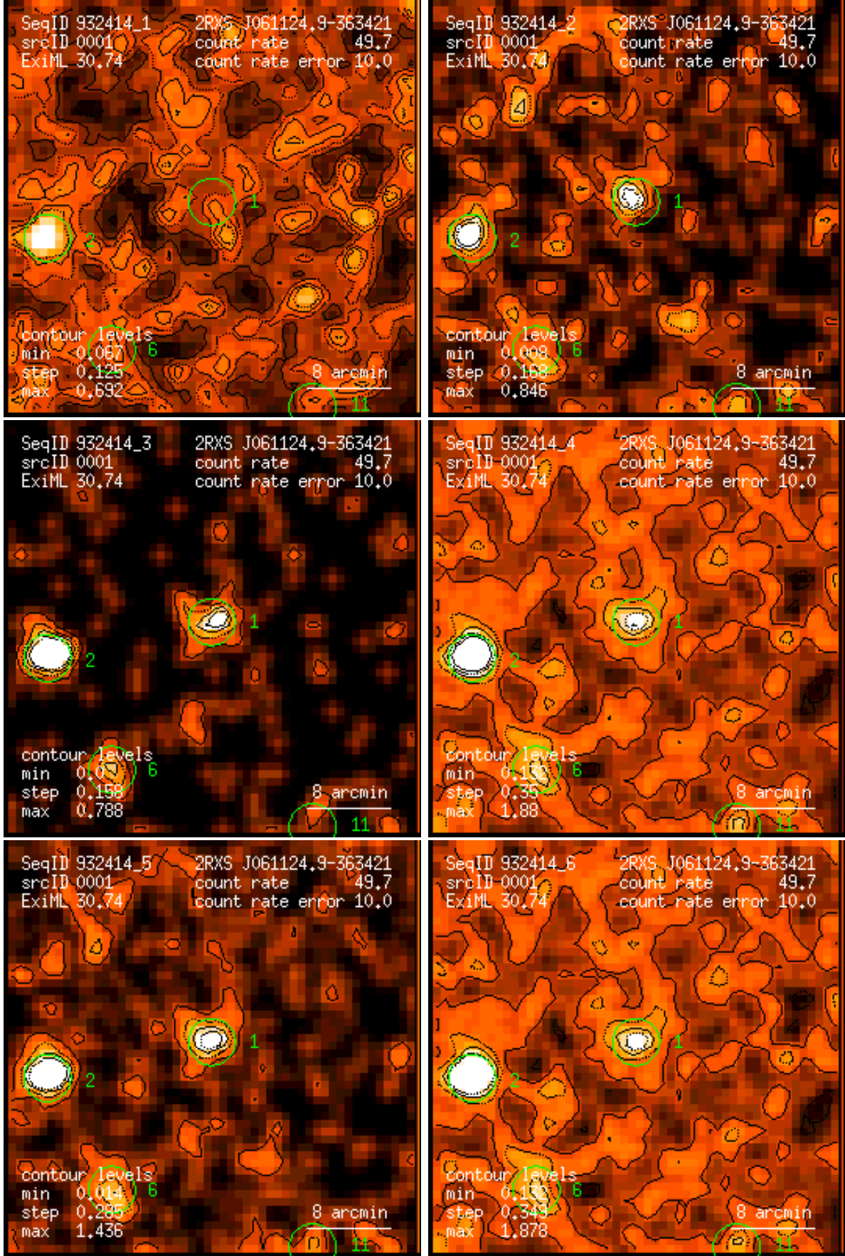
Figure 1: RASS 932414: detection 0001: band rate images, Gaussian filter: (1) PSPC channels 11 – 41, (2) 52 – 90, (3) 91 – 201, (4) 11 – 235, (5) 52 – 201, (6) 11 – 201. Broad band rates in counts/ks. Band rate contour levels in counts/ks/arcmin 2 .
