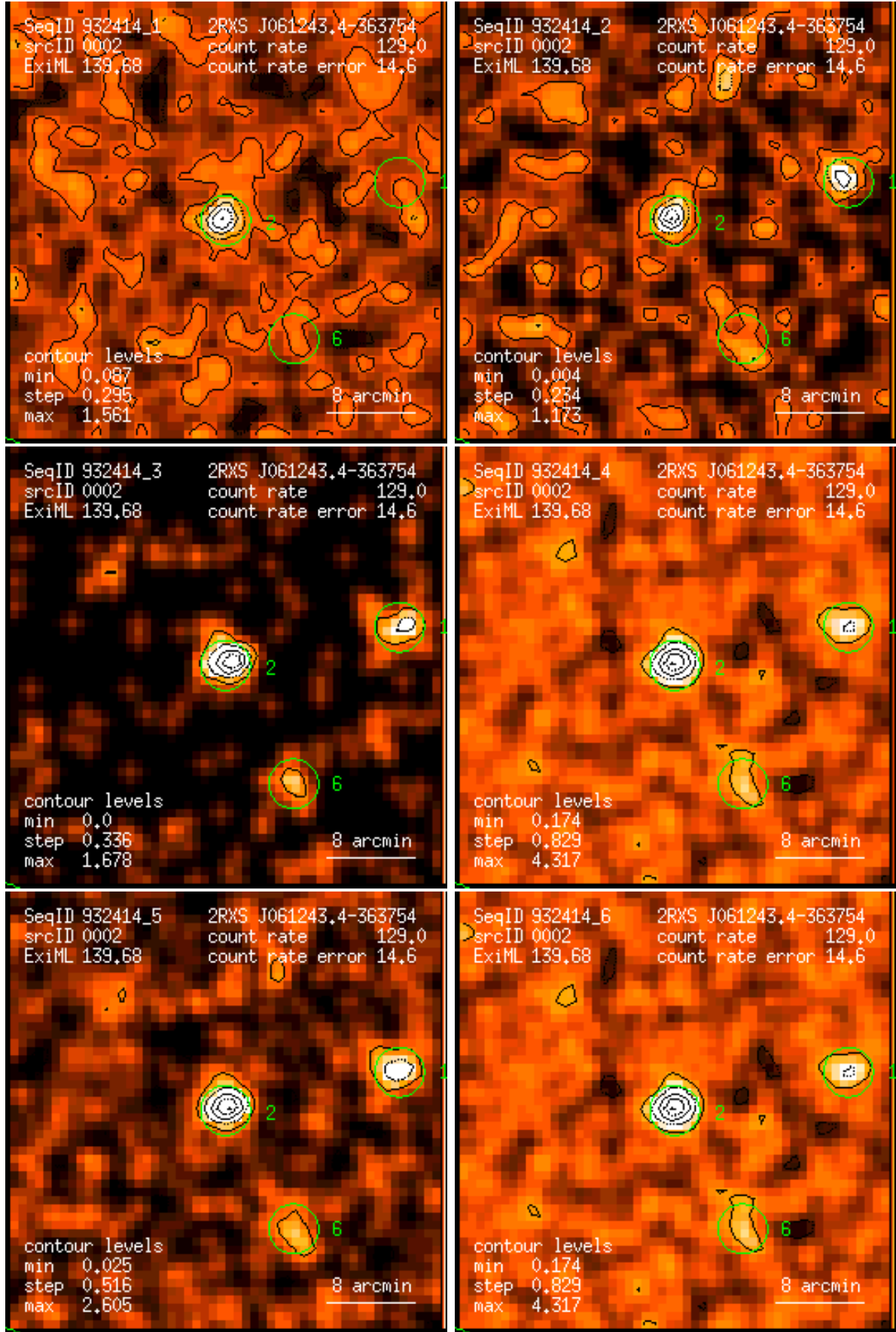
Figure 2: RASS 932414: detection 0002: band rate images, Gaussian filter: (1) PSPC channels 11 – 41, (2) 52 – 90, (3) 91 – 201, (4) 11 – 235, (5) 52 – 201, (6) 11 – 201. Broad band rates in counts/ks. Band rate contour levels in counts/ks/arcmin 2 .
