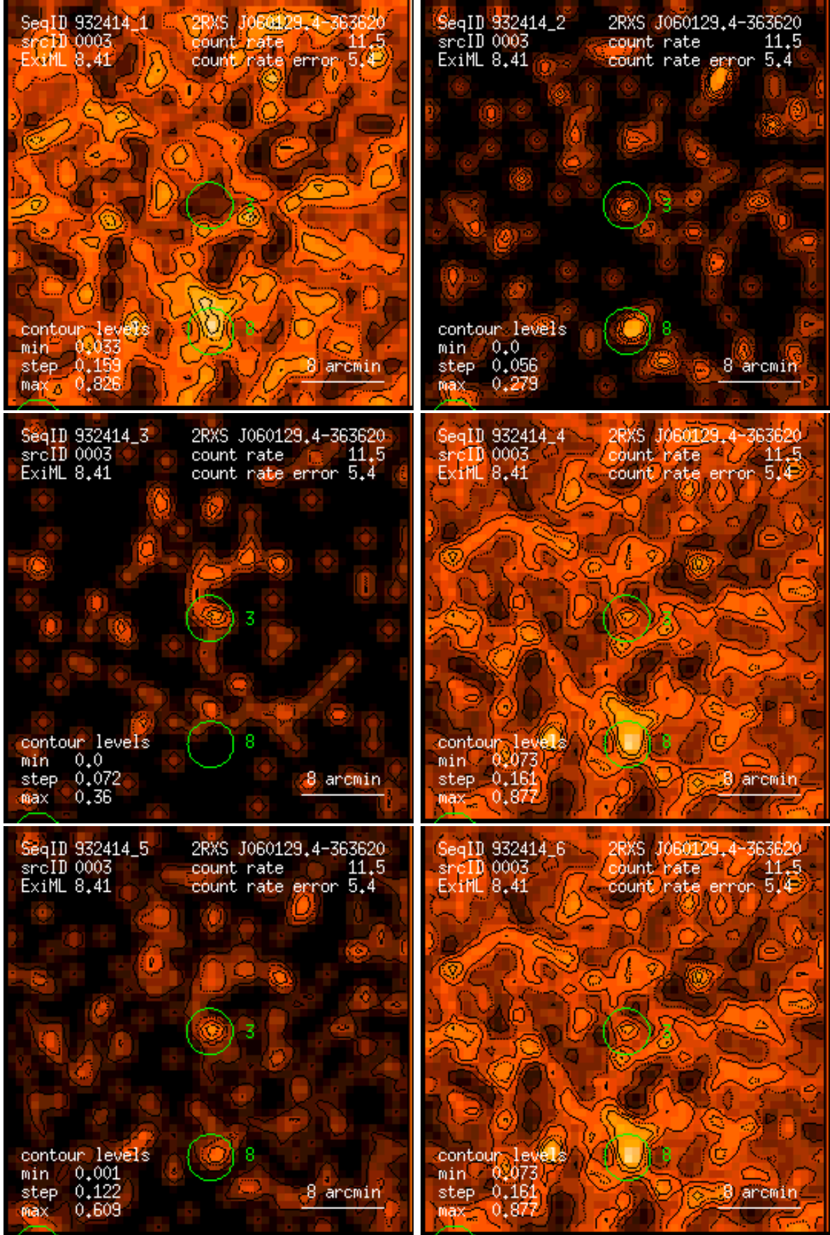
Figure 3: RASS 932414: detection 0003: band rate images, Gaussian filter: (1) PSPC channels 11 – 41, (2) 52 – 90, (3) 91 – 201, (4) 11 – 235, (5) 52 – 201, (6) 11 – 201. Broad band rates in counts/ks. Band rate contour levels in counts/ks/arcmin 2 .
