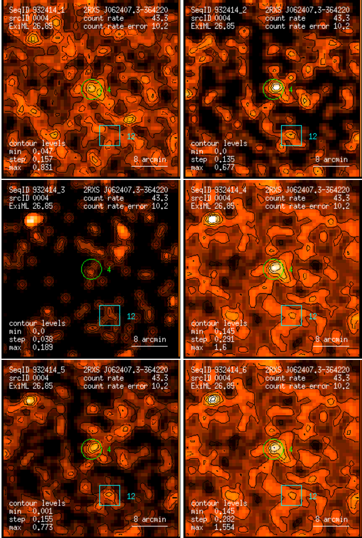
Figure 4: RASS 932414: detection 0004: band rate images, Gaussian filter: (1) PSPC channels 11 – 41, (2) 52 – 90, (3) 91 – 201, (4) 11 – 235, (5) 52 – 201, (6) 11 – 201. Broad band rates in counts/ks. Band rate contour levels in counts/ks/arcmin 2 .
