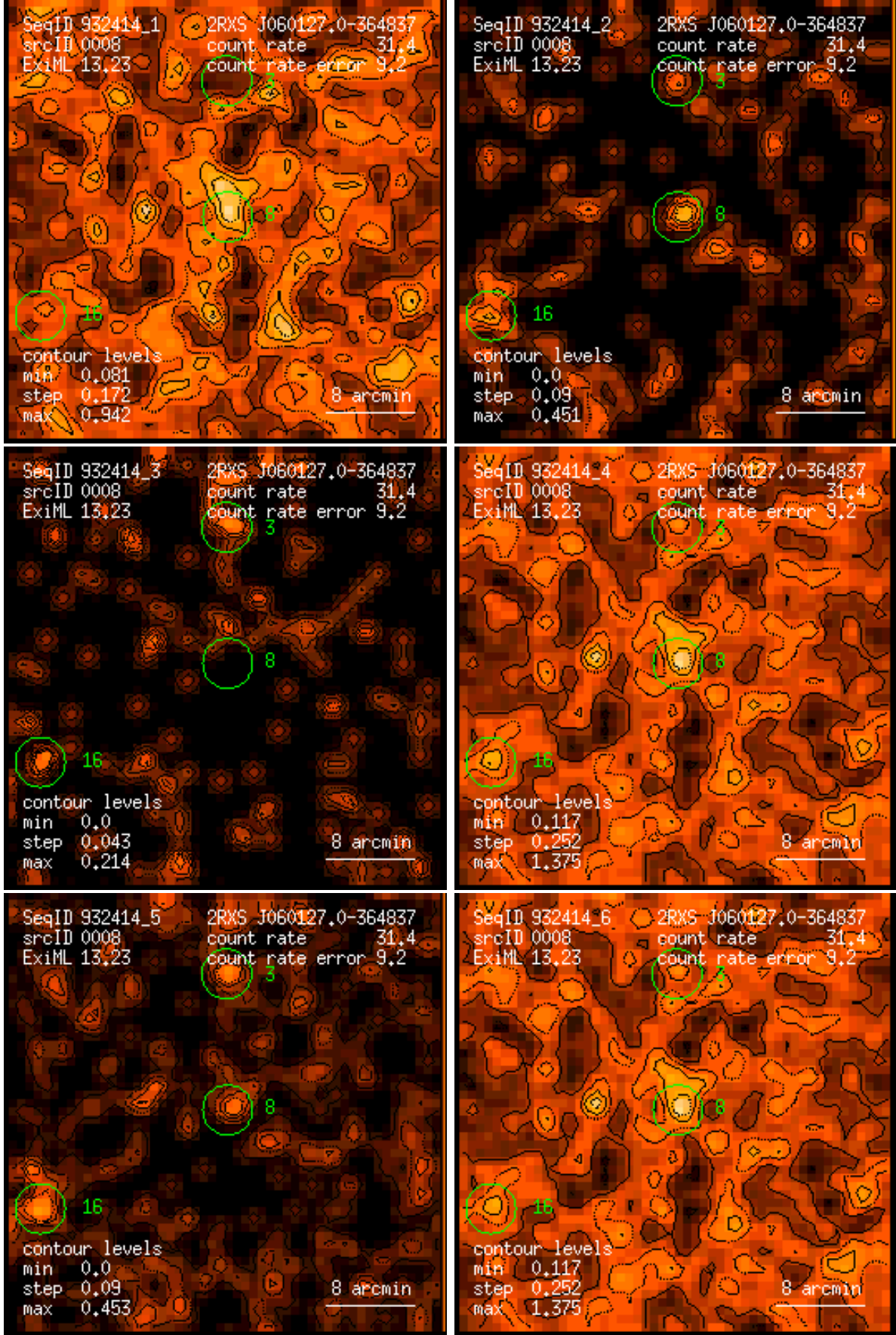
Figure 8: RASS 932414: detection 0008: band rate images, Gaussian filter: (1) PSPC channels 11 – 41, (2) 52 – 90, (3) 91 – 201, (4) 11 – 235, (5) 52 – 201, (6) 11 – 201. Broad band rates in counts/ks. Band rate contour levels in counts/ks/arcmin 2 .
