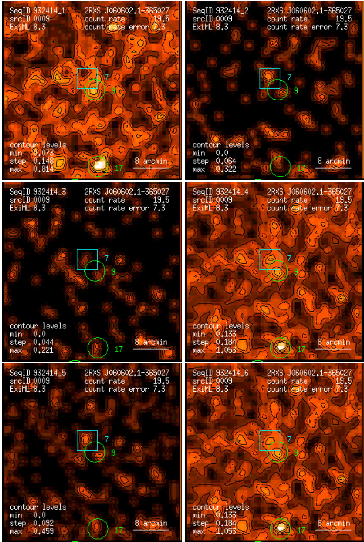
Figure 9: RASS 932414: detection 0009: band rate images, Gaussian filter: (1) PSPC channels 11 – 41, (2) 52 – 90, (3) 91 – 201, (4) 11 – 235, (5) 52 – 201, (6) 11 – 201. Broad band rates in counts/ks. Band rate contour levels in counts/ks/arcmin 2 .
