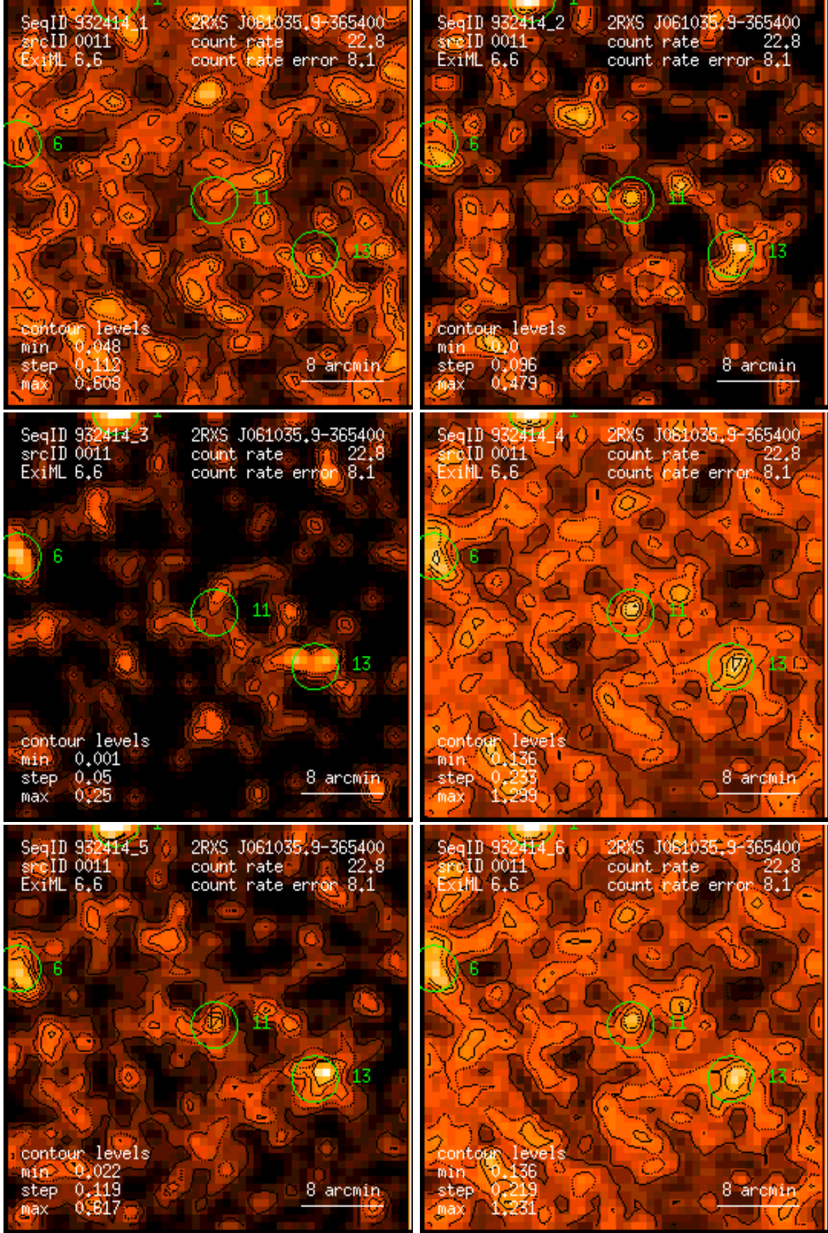
Figure 11: RASS 932414: detection 0011: band rate images, Gaussian filter: (1) PSPC channels 11 – 41, (2) 52 – 90, (3) 91 – 201, (4) 11 – 235, (5) 52 – 201, (6) 11 – 201. Broad band rates in counts/ks. Band rate contour levels in counts/ks/arcmin 2 .
