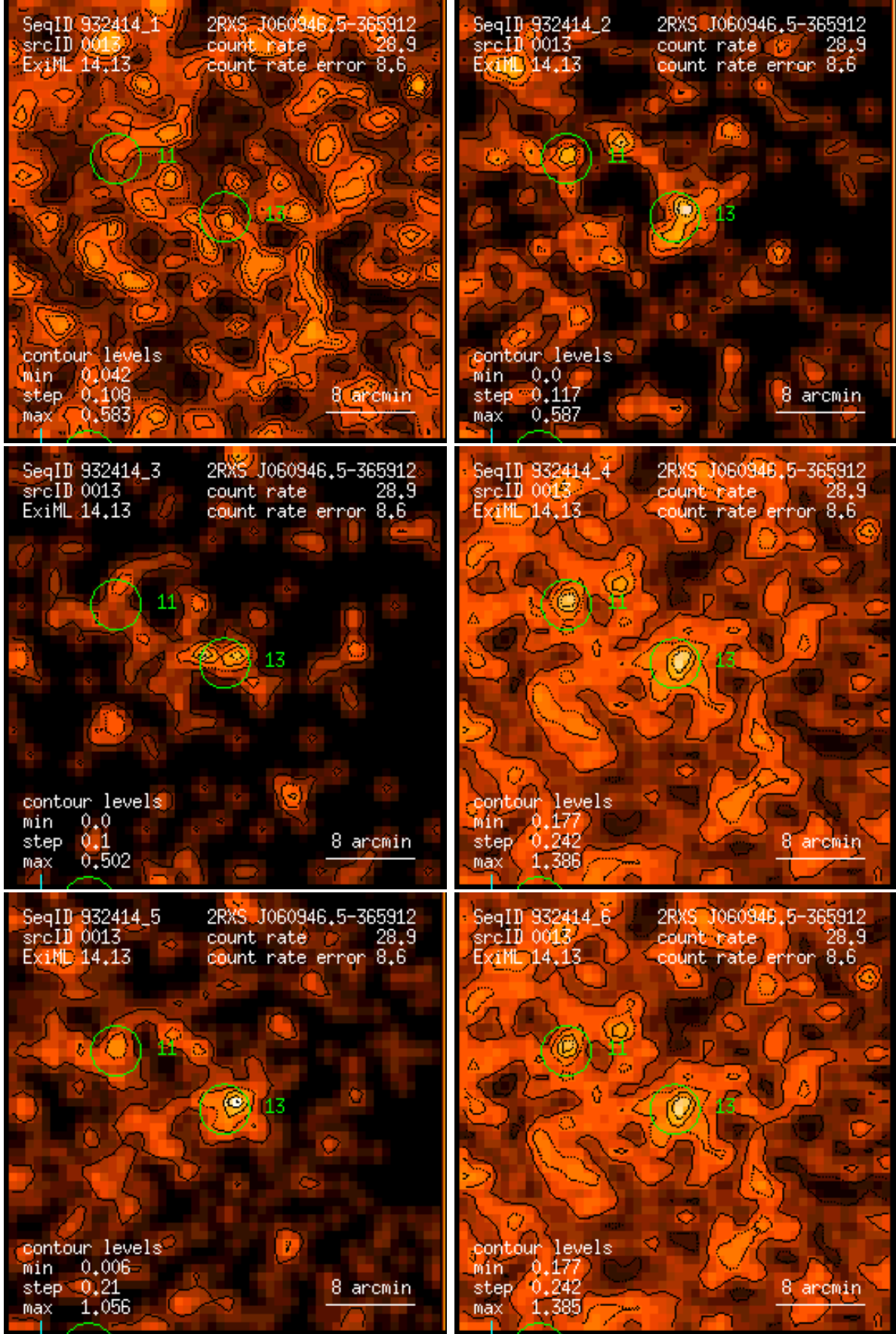
Figure 13: RASS 932414: detection 0013: band rate images, Gaussian filter: (1) PSPC channels 11 – 41, (2) 52 – 90, (3) 91 – 201, (4) 11 – 235, (5) 52 – 201, (6) 11 – 201. Broad band rates in counts/ks. Band rate contour levels in counts/ks/arcmin 2 .
