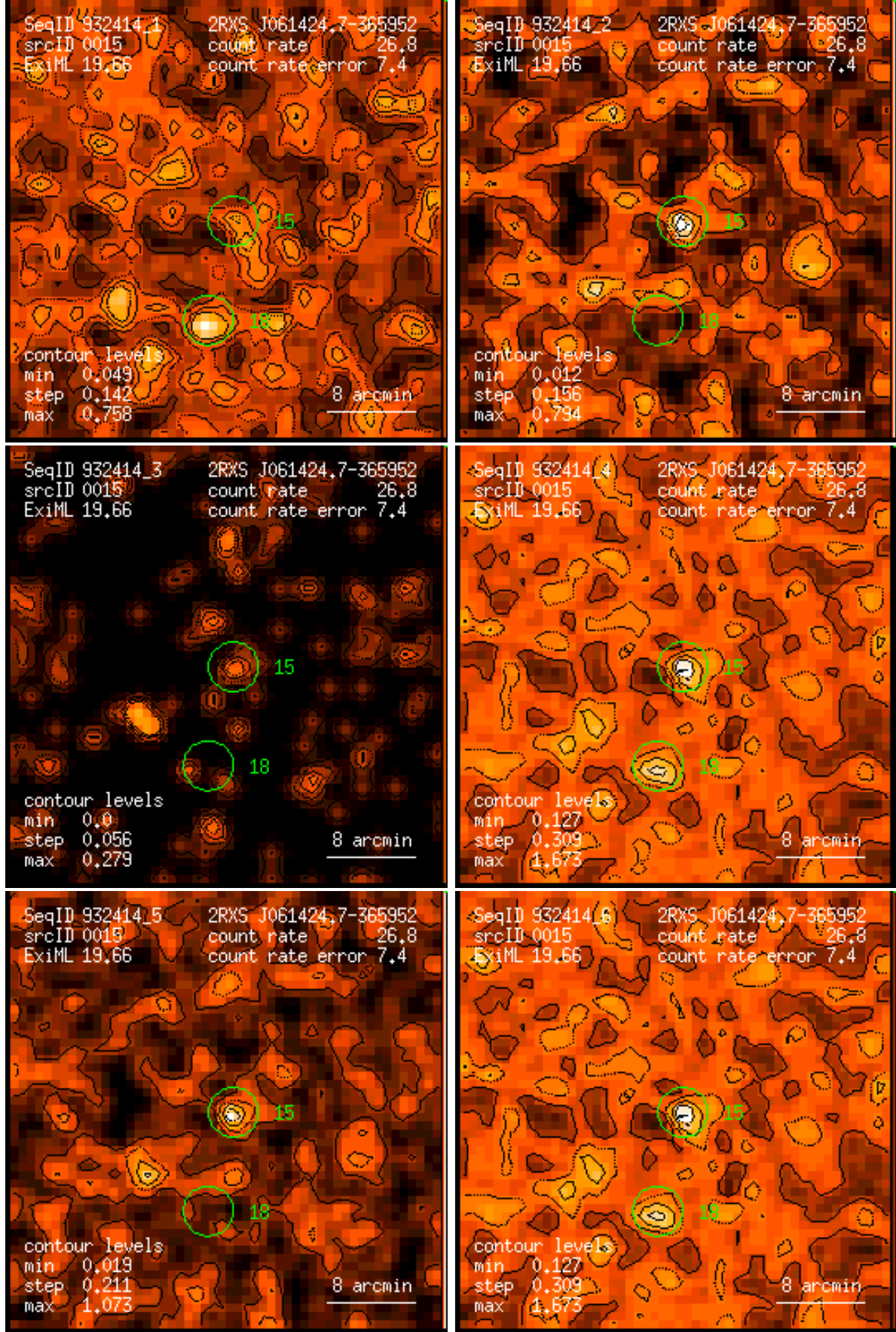
Figure 15: RASS 932414: detection 0015: band rate images, Gaussian filter: (1) PSPC channels 11 – 41, (2) 52 – 90, (3) 91 – 201, (4) 11 – 235, (5) 52 – 201, (6) 11 – 201. Broad band rates in counts/ks. Band rate contour levels in counts/ks/arcmin 2 .
