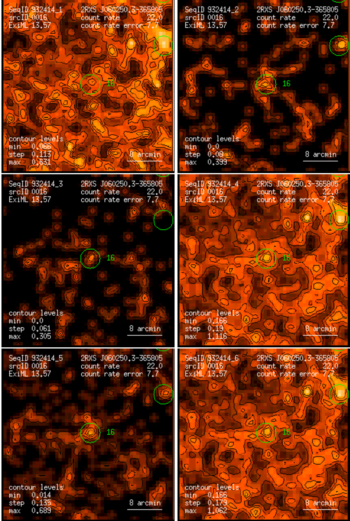
Figure 16: RASS 932414: detection 0016: band rate images, Gaussian filter: (1) PSPC channels 11 – 41, (2) 52 – 90, (3) 91 – 201, (4) 11 – 235, (5) 52 – 201, (6) 11 – 201. Broad band rates in counts/ks. Band rate contour levels in counts/ks/arcmin 2 .
