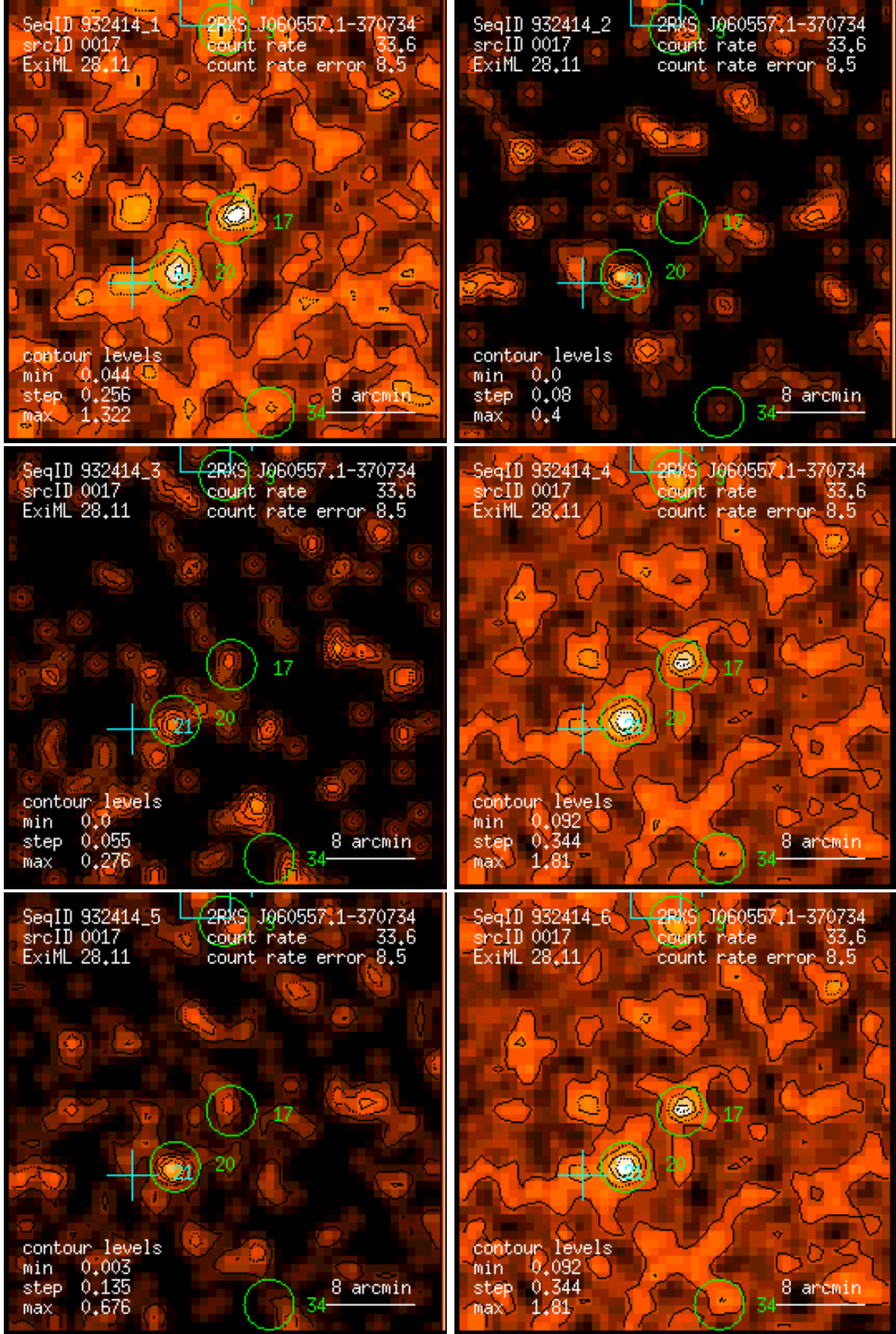
Figure 17: RASS 932414: detection 0017: band rate images, Gaussian filter: (1) PSPC channels 11 – 41, (2) 52 – 90, (3) 91 – 201, (4) 11 – 235, (5) 52 – 201, (6) 11 – 201. Broad band rates in counts/ks. Band rate contour levels in counts/ks/arcmin 2 .
