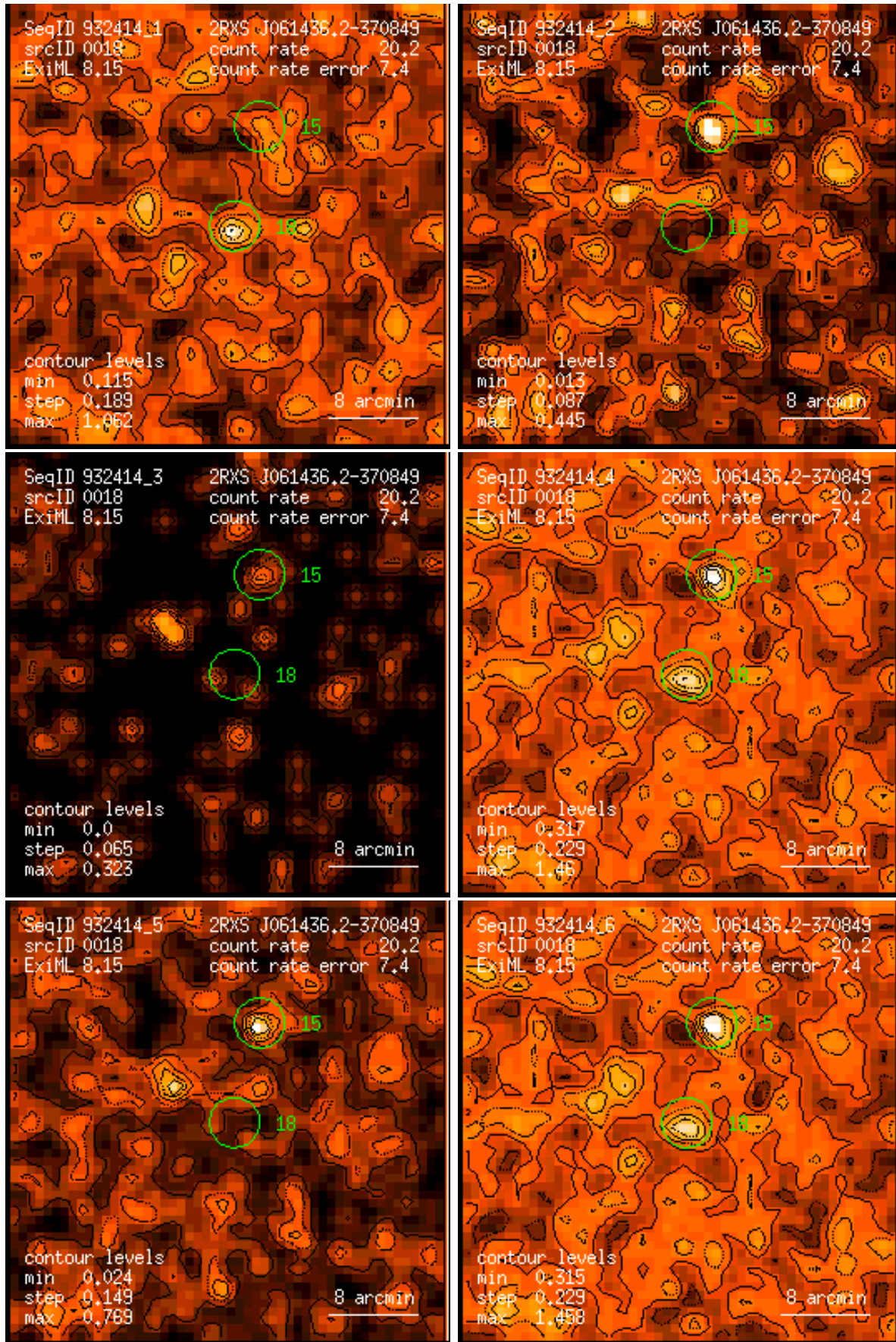
Figure 18: RASS 932414: detection 0018: band rate images, Gaussian filter: (1) PSPC channels 11 – 41, (2) 52 – 90, (3) 91 – 201, (4) 11 – 235, (5) 52 – 201, (6) 11 – 201. Broad band rates in counts/ks. Band rate contour levels in counts/ks/arcmin 2 .
