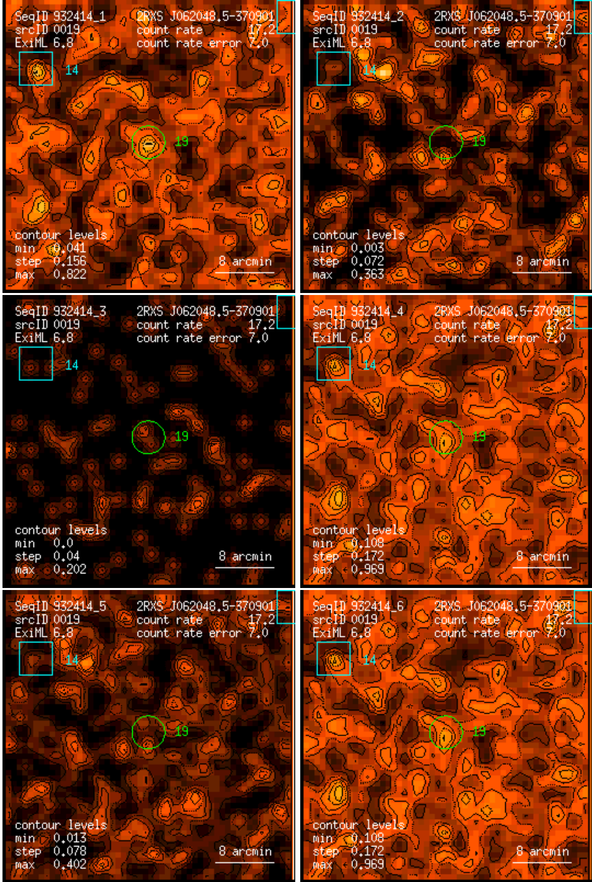
Figure 19: RASS 932414: detection 0019: band rate images, Gaussian filter: (1) PSPC channels 11 – 41, (2) 52 – 90, (3) 91 – 201, (4) 11 – 235, (5) 52 – 201, (6) 11 – 201. Broad band rates in counts/ks. Band rate contour levels in counts/ks/arcmin 2 .
