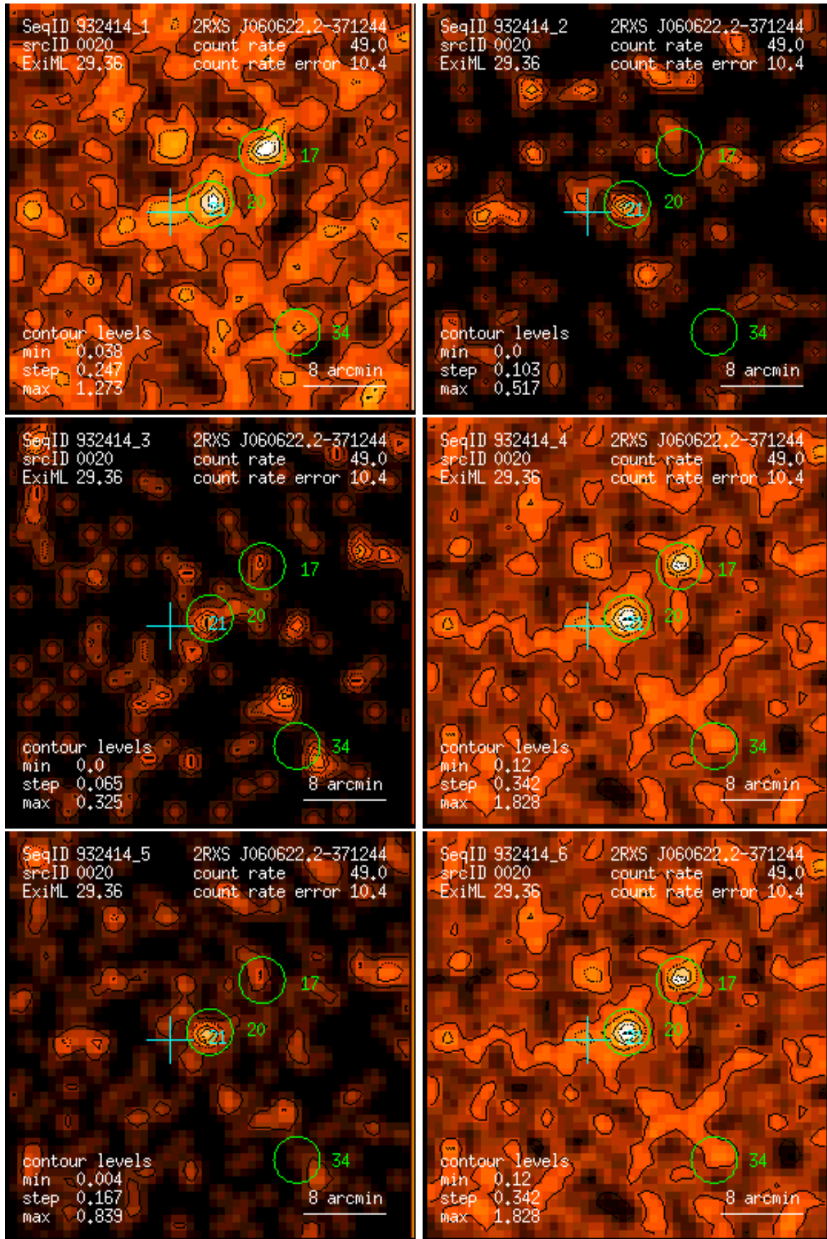
Figure 20: RASS 932414: detection 0020: band rate images, Gaussian filter: (1) PSPC channels 11 – 41, (2) 52 – 90, (3) 91 – 201, (4) 11 – 235, (5) 52 – 201, (6) 11 – 201. Broad band rates in counts/ks. Band rate contour levels in counts/ks/arcmin 2 .
