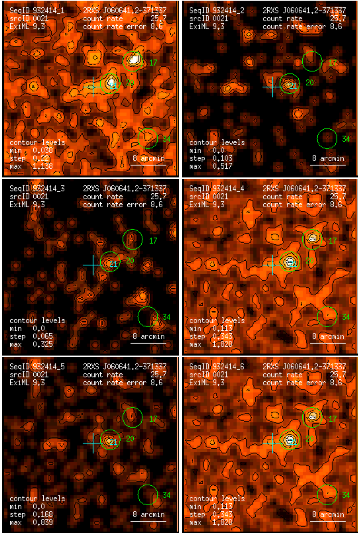
Figure 21: RASS 932414: detection 0021: band rate images, Gaussian filter: (1) PSPC channels 11 – 41, (2) 52 – 90, (3) 91 – 201, (4) 11 – 235, (5) 52 – 201, (6) 11 – 201. Broad band rates in counts/ks. Band rate contour levels in counts/ks/arcmin 2 .
