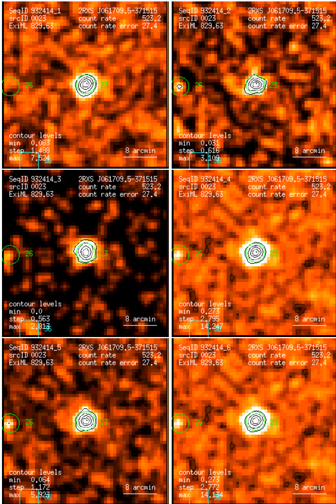
Figure 23: RASS 932414: detection 0023: band rate images, Gaussian filter: (1) PSPC channels 11 – 41, (2) 52 – 90, (3) 91 – 201, (4) 11 – 235, (5) 52 – 201, (6) 11 – 201. Broad band rates in counts/ks. Band rate contour levels in counts/ks/arcmin 2 .
