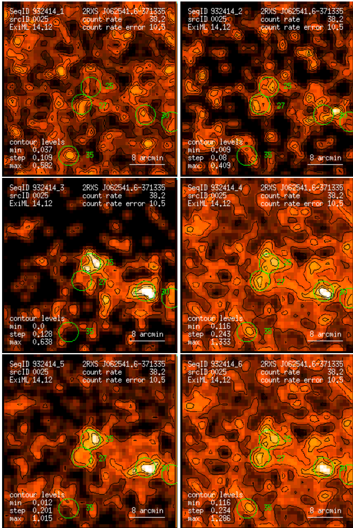
Figure 25: RASS 932414: detection 0025: band rate images, Gaussian filter: (1) PSPC channels 11 – 41, (2) 52 – 90, (3) 91 – 201, (4) 11 – 235, (5) 52 – 201, (6) 11 – 201. Broad band rates in counts/ks. Band rate contour levels in counts/ks/arcmin 2 .
