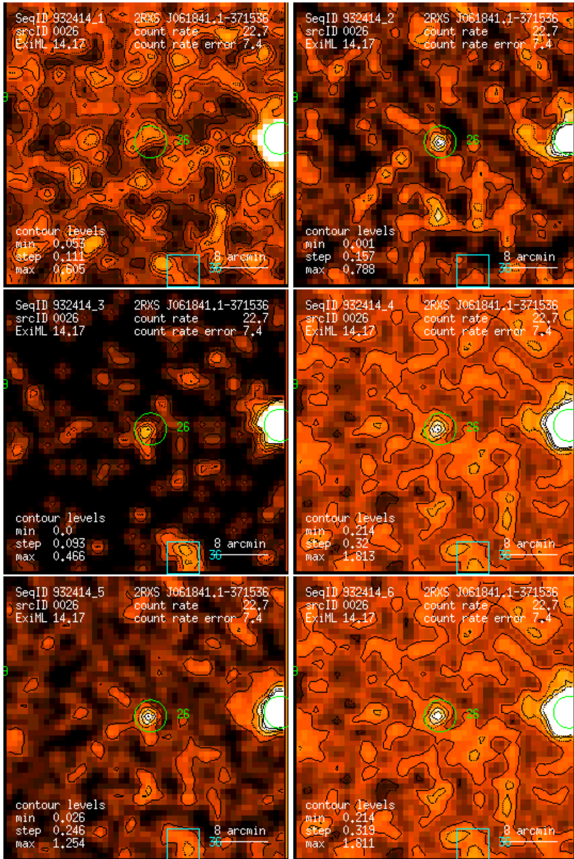
Figure 26: RASS 932414: detection 0026: band rate images, Gaussian filter: (1) PSPC channels 11 – 41, (2) 52 – 90, (3) 91 – 201, (4) 11 – 235, (5) 52 – 201, (6) 11 – 201. Broad band rates in counts/ks. Band rate contour levels in counts/ks/arcmin 2 .
