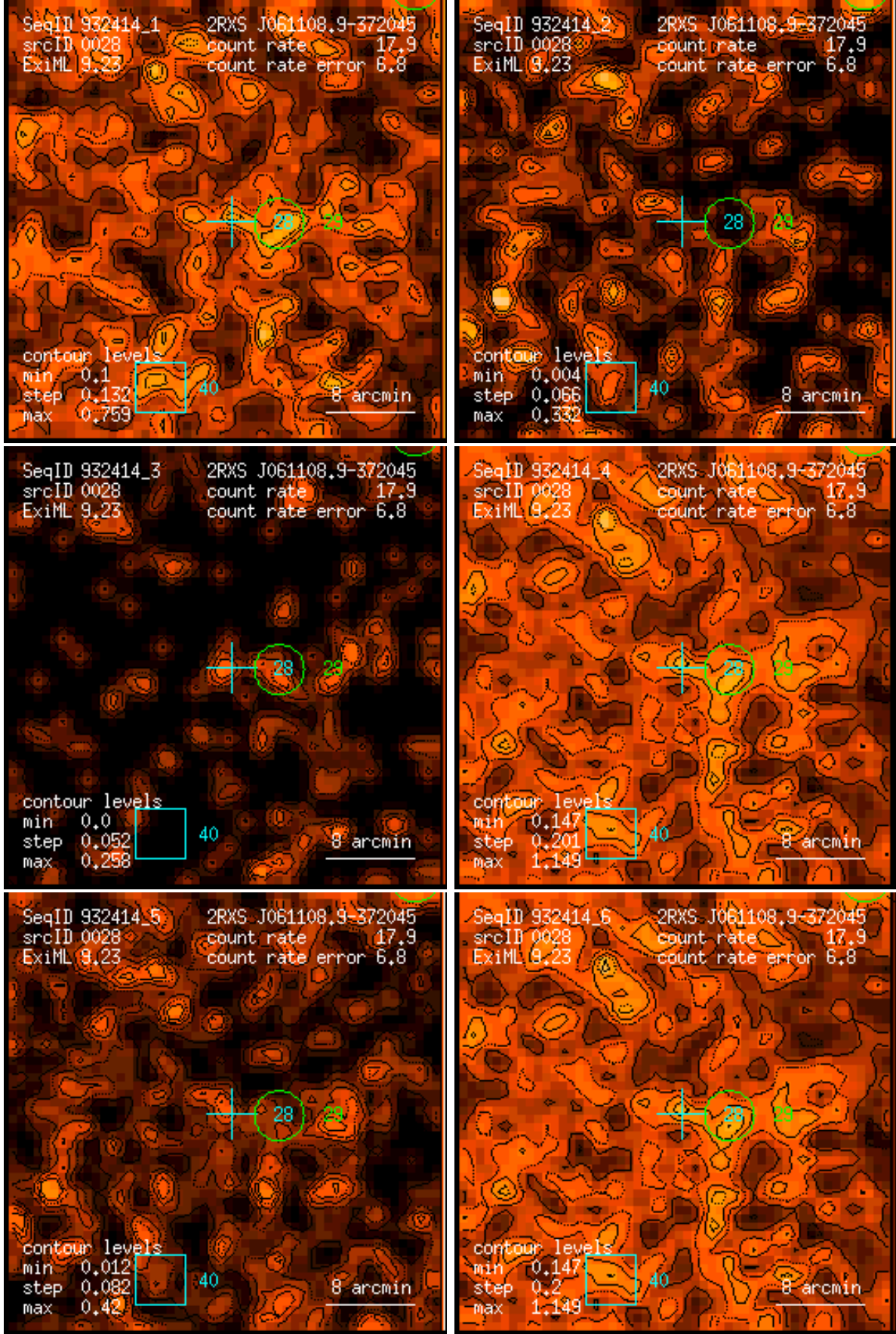
Figure 28: RASS 932414: detection 0028: band rate images, Gaussian filter: (1) PSPC channels 11 – 41, (2) 52 – 90, (3) 91 – 201, (4) 11 – 235, (5) 52 – 201, (6) 11 – 201. Broad band rates in counts/ks. Band rate contour levels in counts/ks/arcmin 2 .
