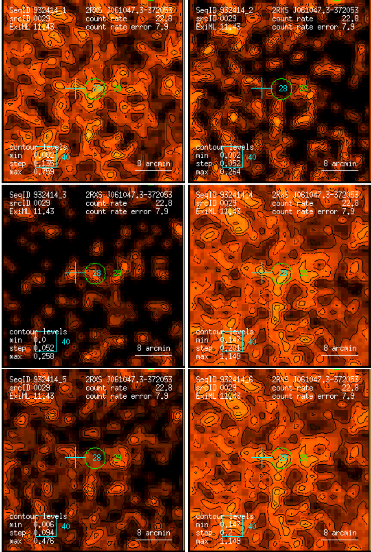
Figure 29: RASS 932414: detection 0029: band rate images, Gaussian filter: (1) PSPC channels 11 – 41, (2) 52 – 90, (3) 91 – 201, (4) 11 – 235, (5) 52 – 201, (6) 11 – 201. Broad band rates in counts/ks. Band rate contour levels in counts/ks/arcmin 2 .
