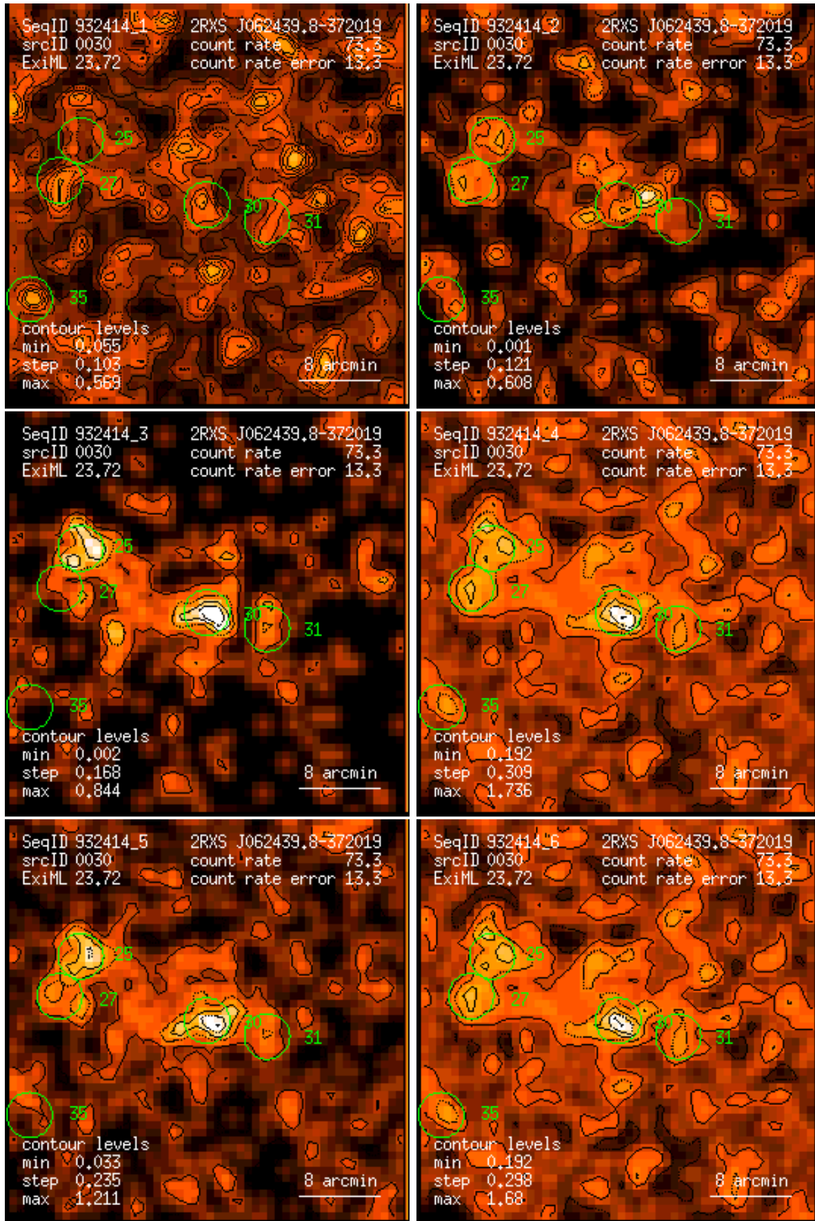
Figure 30: RASS 932414: detection 0030: band rate images, Gaussian filter: (1) PSPC channels 11 – 41, (2) 52 – 90, (3) 91 – 201, (4) 11 – 235, (5) 52 – 201, (6) 11 – 201. Broad band rates in counts/ks. Band rate contour levels in counts/ks/arcmin 2 .
