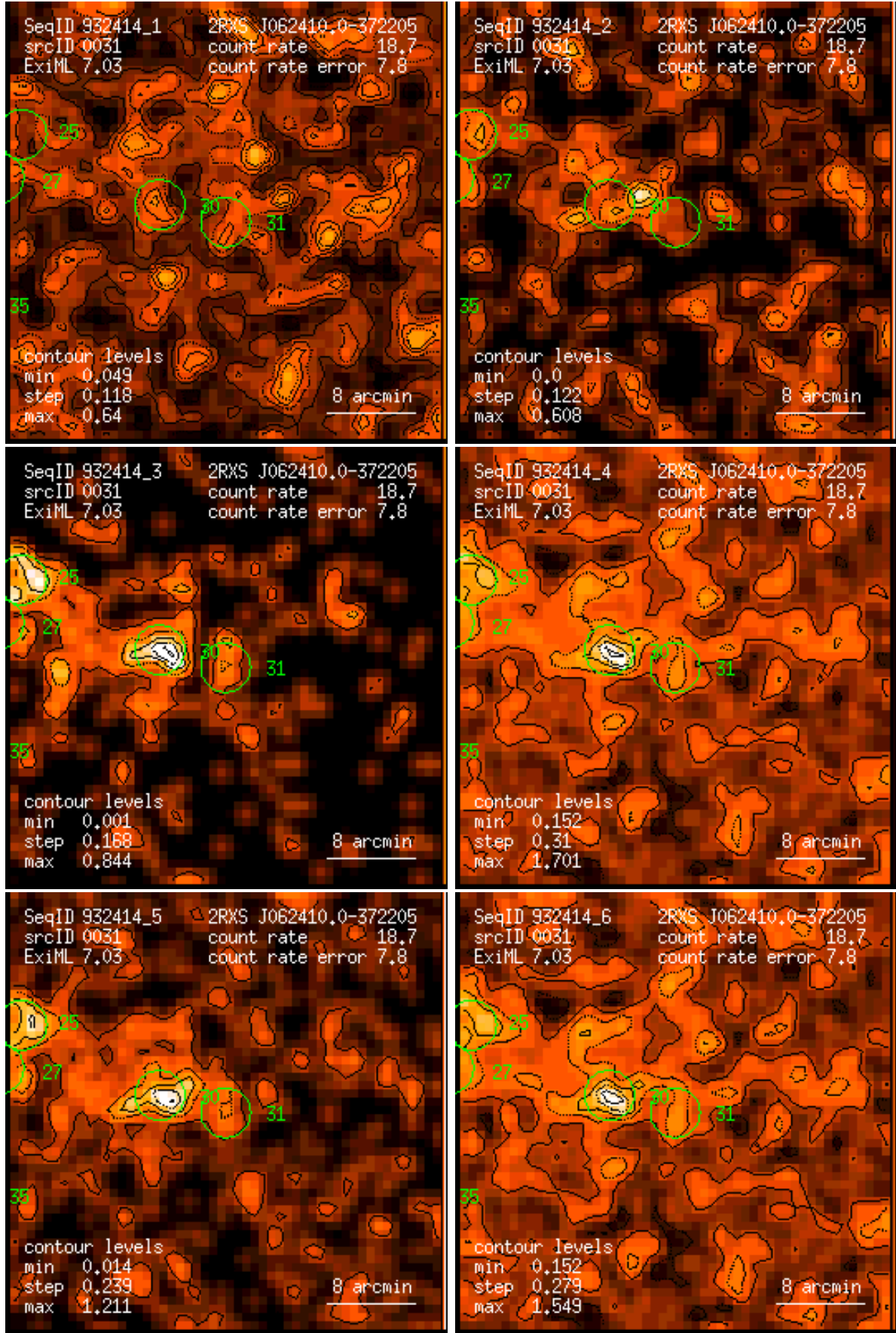
Figure 31: RASS 932414: detection 0031: band rate images, Gaussian filter: (1) PSPC channels 11 – 41, (2) 52 – 90, (3) 91 – 201, (4) 11 – 235, (5) 52 – 201, (6) 11 – 201. Broad band rates in counts/ks. Band rate contour levels in counts/ks/arcmin 2 .
