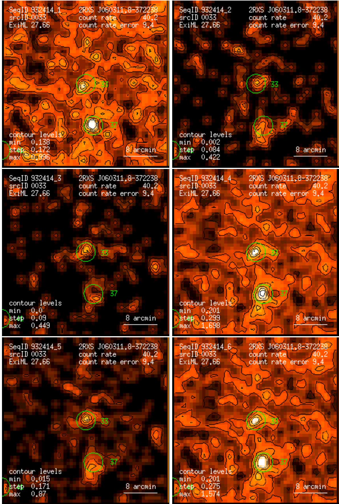
Figure 33: RASS 932414: detection 0033: band rate images, Gaussian filter: (1) PSPC channels 11 – 41, (2) 52 – 90, (3) 91 – 201, (4) 11 – 235, (5) 52 – 201, (6) 11 – 201. Broad band rates in counts/ks. Band rate contour levels in counts/ks/arcmin 2 .
