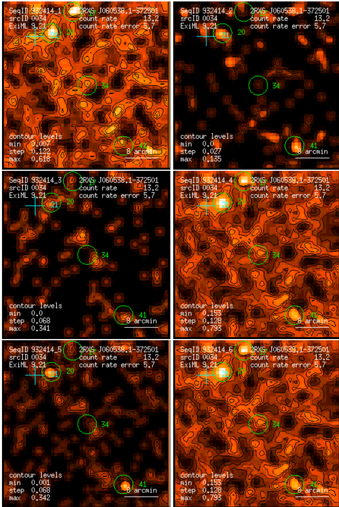
Figure 34: RASS 932414: detection 0034: band rate images, Gaussian filter: (1) PSPC channels 11 – 41, (2) 52 – 90, (3) 91 – 201, (4) 11 – 235, (5) 52 – 201, (6) 11 – 201. Broad band rates in counts/ks. Band rate contour levels in counts/ks/arcmin 2 .
