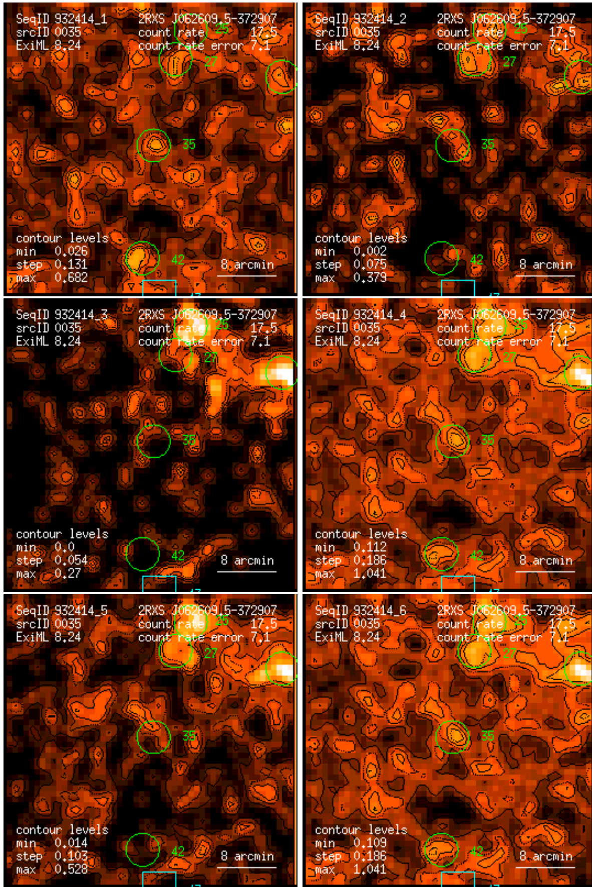
Figure 35: RASS 932414: detection 0035: band rate images, Gaussian filter: (1) PSPC channels 11 – 41, (2) 52 – 90, (3) 91 – 201, (4) 11 – 235, (5) 52 – 201, (6) 11 – 201. Broad band rates in counts/ks. Band rate contour levels in counts/ks/arcmin 2 .
