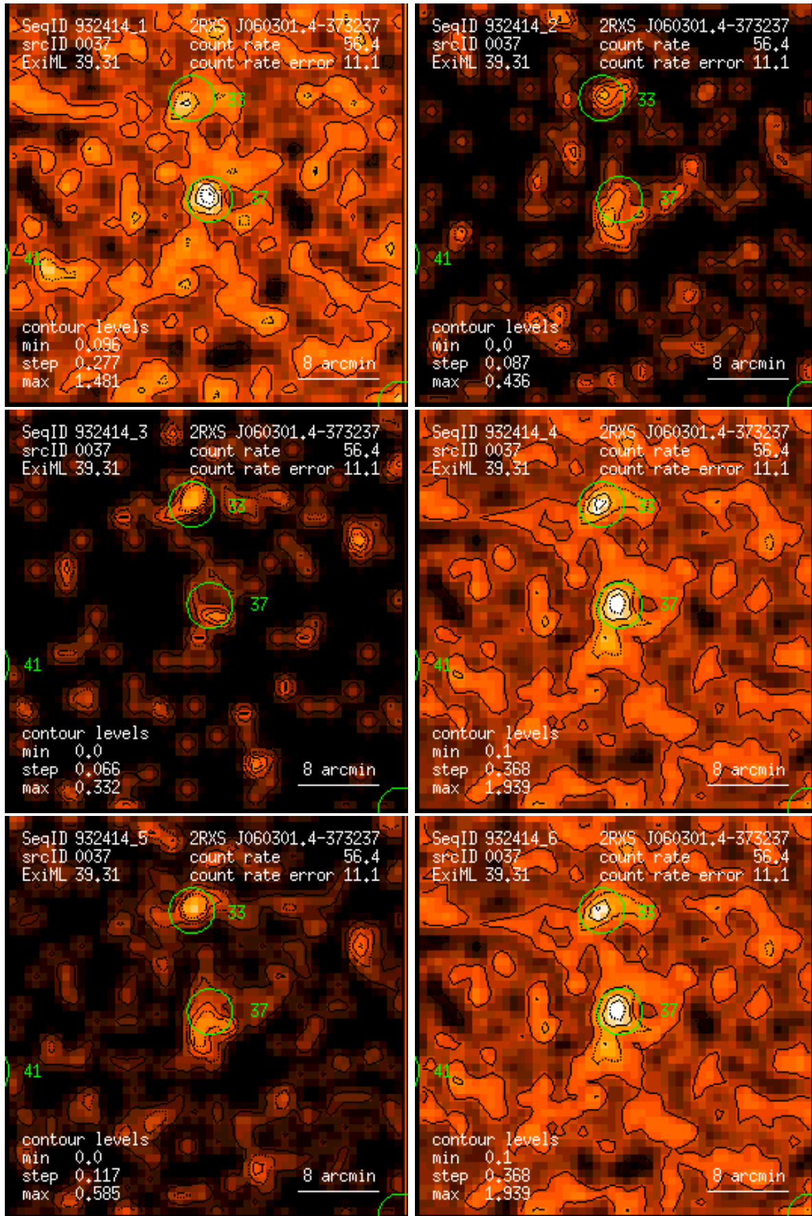
Figure 37: RASS 932414: detection 0037: band rate images, Gaussian filter: (1) PSPC channels 11 – 41, (2) 52 – 90, (3) 91 – 201, (4) 11 – 235, (5) 52 – 201, (6) 11 – 201. Broad band rates in counts/ks. Band rate contour levels in counts/ks/arcmin 2 .
