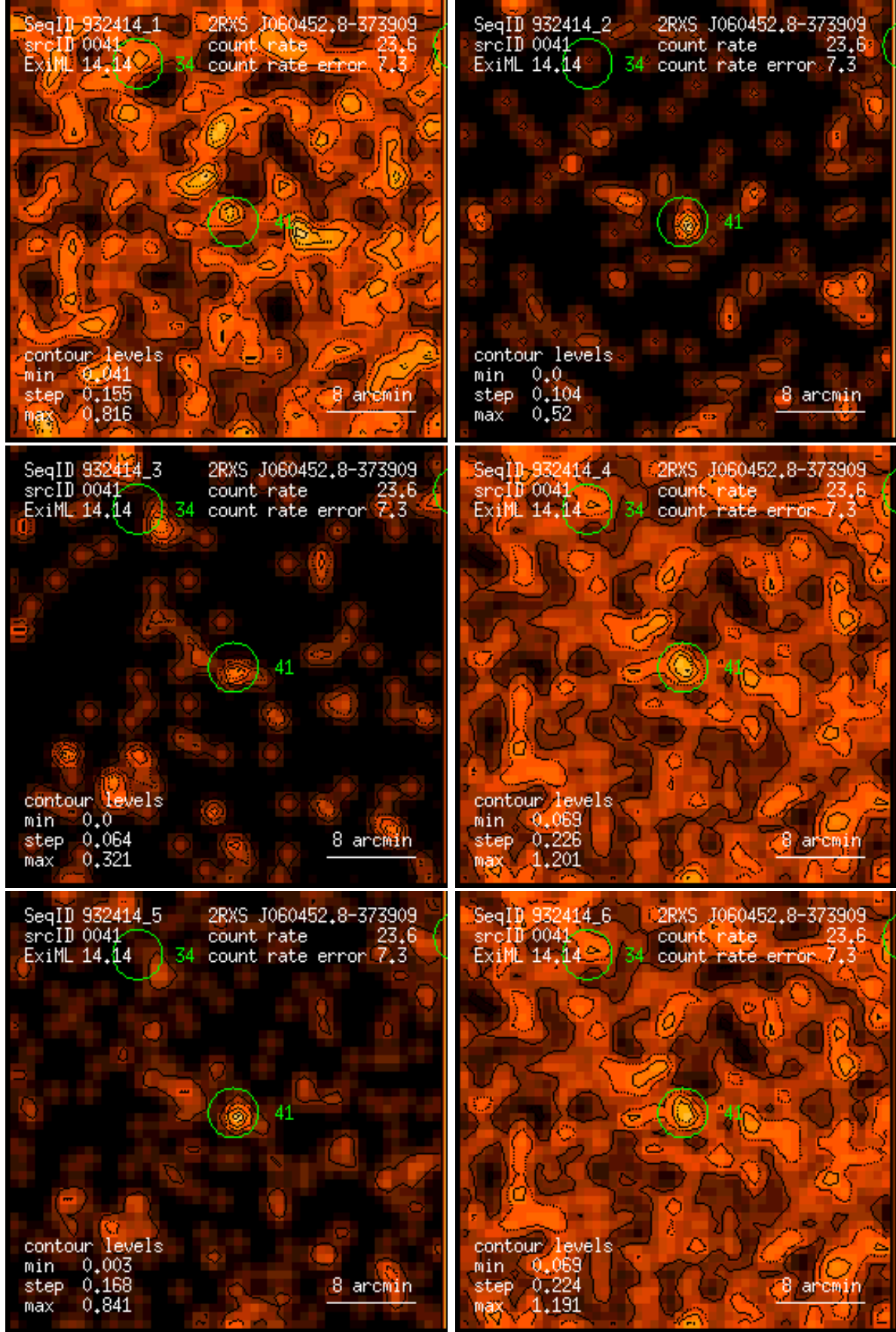
Figure 41: RASS 932414: detection 0041: band rate images, Gaussian filter: (1) PSPC channels 11 – 41, (2) 52 – 90, (3) 91 – 201, (4) 11 – 235, (5) 52 – 201, (6) 11 – 201. Broad band rates in counts/ks. Band rate contour levels in counts/ks/arcmin 2 .
