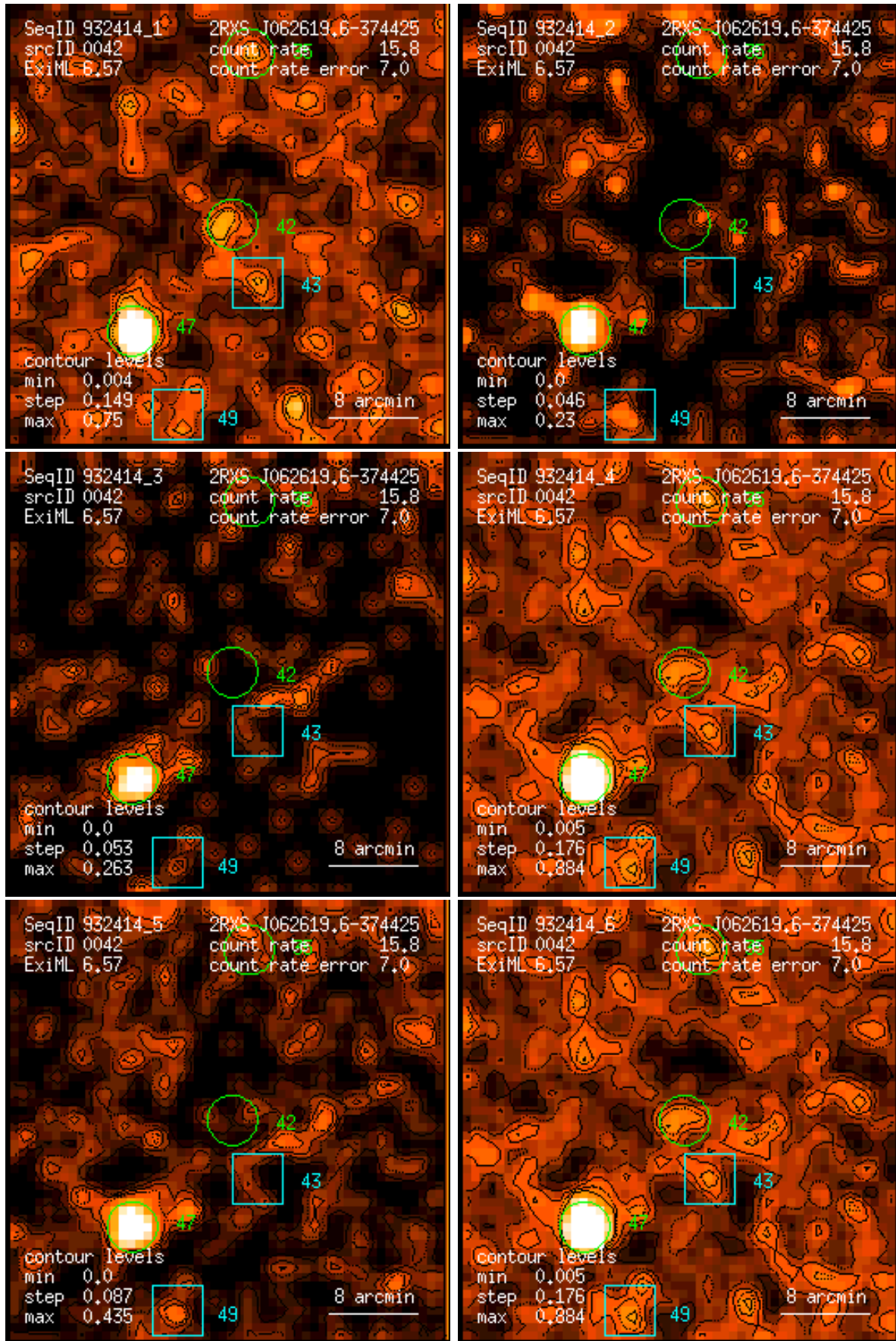
Figure 42: RASS 932414: detection 0042: band rate images, Gaussian filter: (1) PSPC channels 11 – 41, (2) 52 – 90, (3) 91 – 201, (4) 11 – 235, (5) 52 – 201, (6) 11 – 201. Broad band rates in counts/ks. Band rate contour levels in counts/ks/arcmin 2 .
