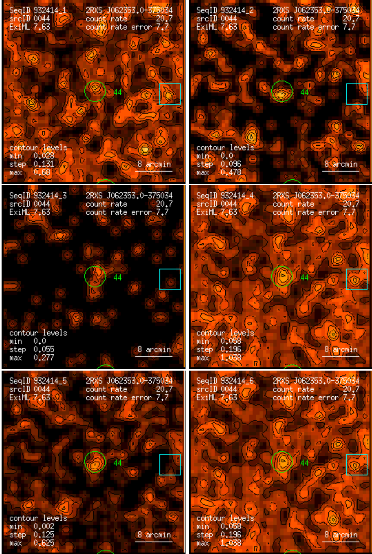
Figure 44: RASS 932414: detection 0044: band rate images, Gaussian filter: (1) PSPC channels 11 – 41, (2) 52 – 90, (3) 91 – 201, (4) 11 – 235, (5) 52 – 201, (6) 11 – 201. Broad band rates in counts/ks. Band rate contour levels in counts/ks/arcmin 2 .
