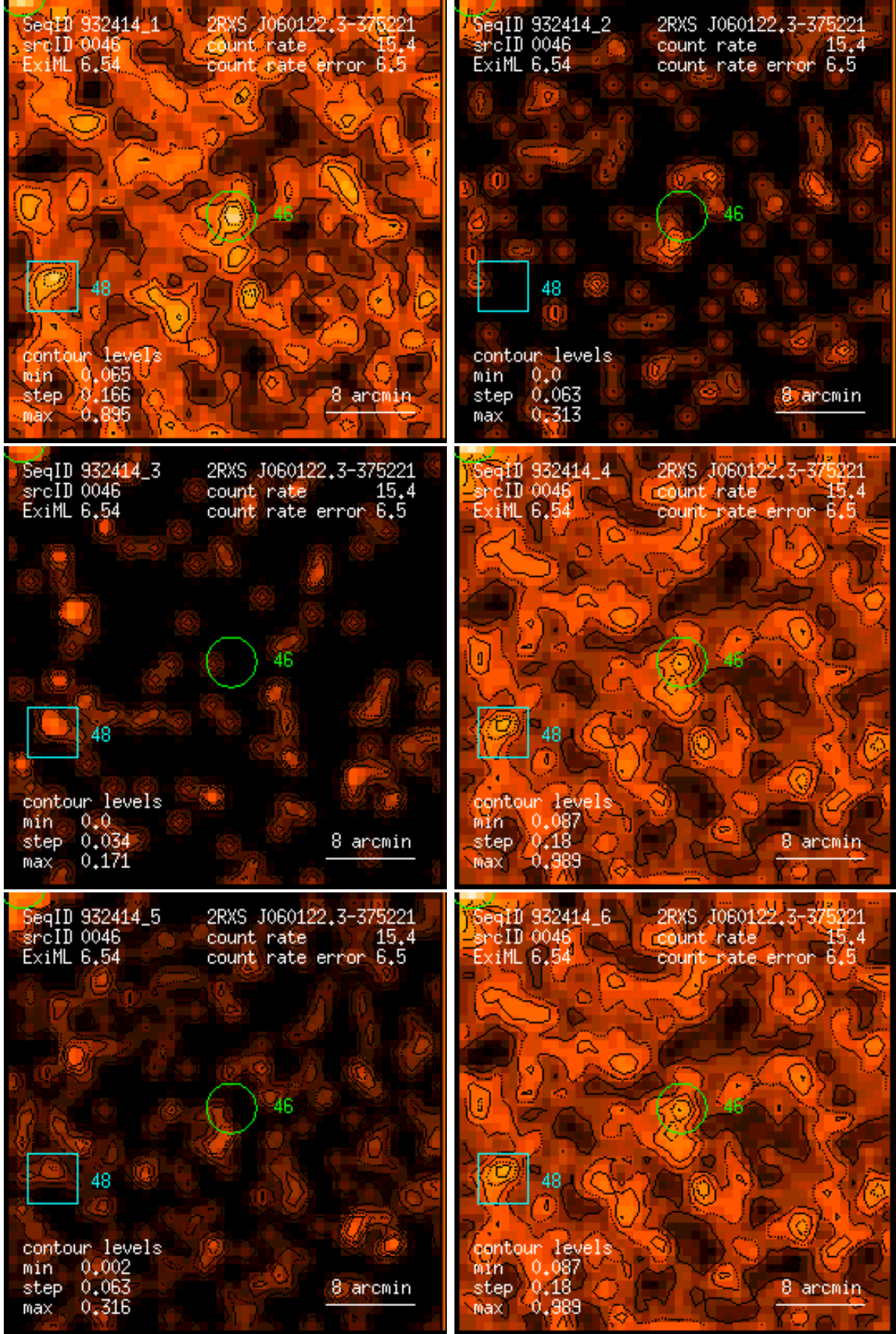
Figure 46: RASS 932414: detection 0046: band rate images, Gaussian filter: (1) PSPC channels 11 – 41, (2) 52 – 90, (3) 91 – 201, (4) 11 – 235, (5) 52 – 201, (6) 11 – 201. Broad band rates in counts/ks. Band rate contour levels in counts/ks/arcmin 2 .
