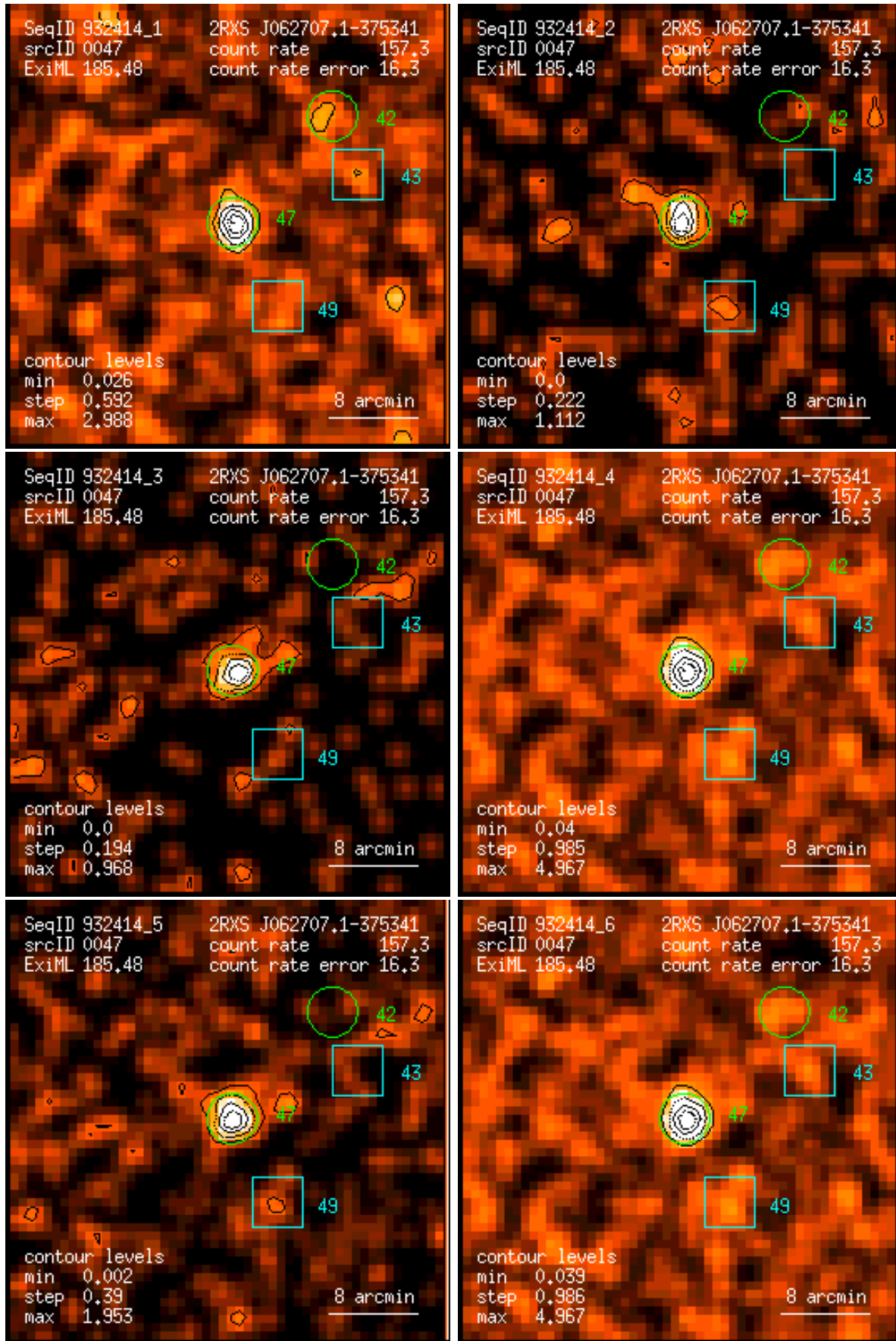
Figure 47: RASS 932414: detection 0047: band rate images, Gaussian filter: (1) PSPC channels 11 – 41, (2) 52 – 90, (3) 91 – 201, (4) 11 – 235, (5) 52 – 201, (6) 11 – 201. Broad band rates in counts/ks. Band rate contour levels in counts/ks/arcmin 2 .
