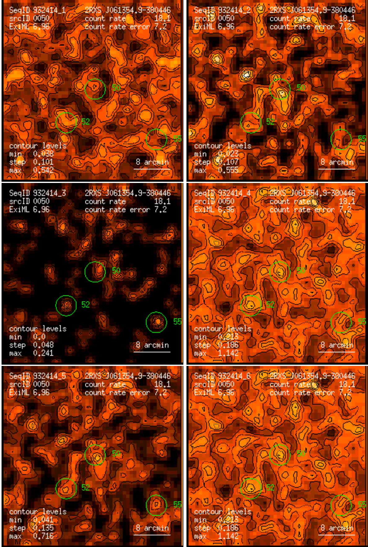
Figure 50: RASS 932414: detection 0050: band rate images, Gaussian filter: (1) PSPC channels 11 – 41, (2) 52 – 90, (3) 91 – 201, (4) 11 – 235, (5) 52 – 201, (6) 11 – 201. Broad band rates in counts/ks. Band rate contour levels in counts/ks/arcmin 2 .
