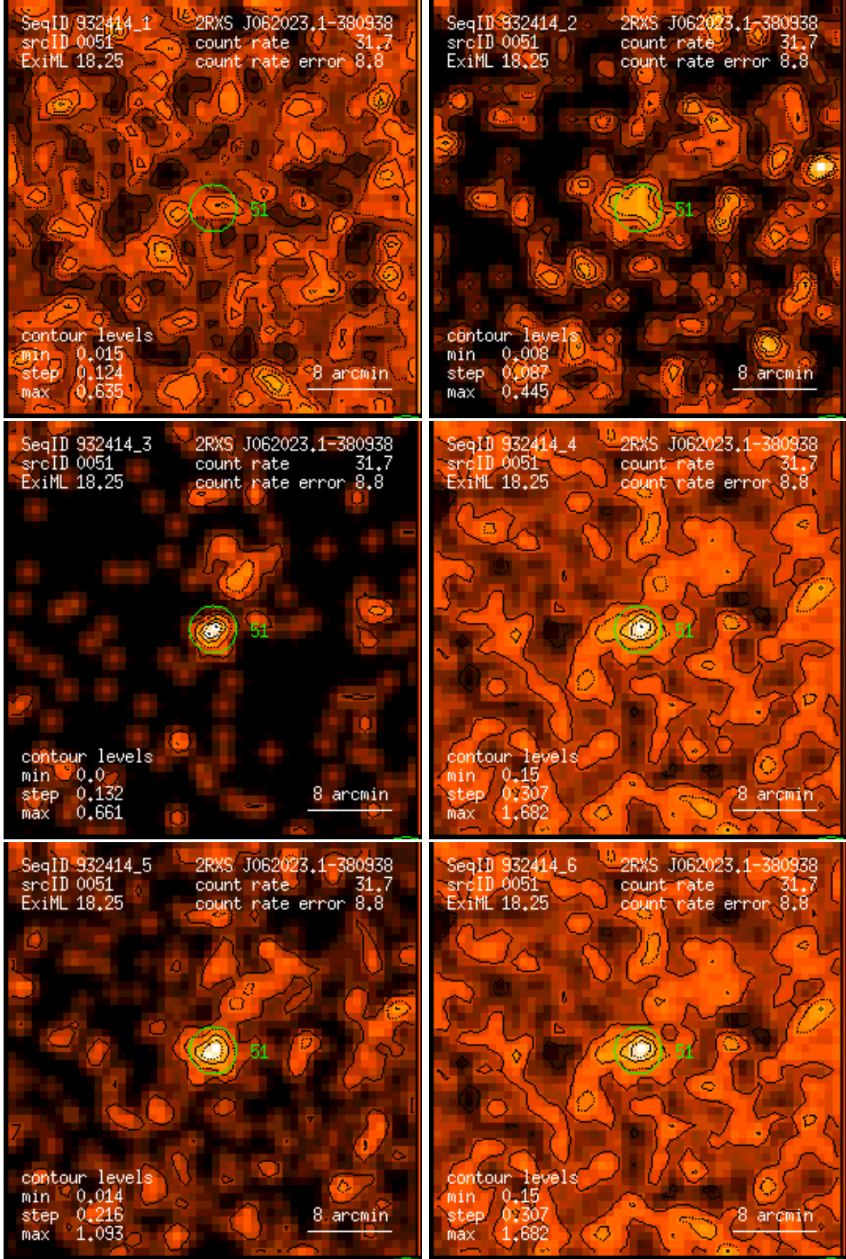
Figure 51: RASS 932414: detection 0051: band rate images, Gaussian filter: (1) PSPC channels 11 – 41, (2) 52 – 90, (3) 91 – 201, (4) 11 – 235, (5) 52 – 201, (6) 11 – 201. Broad band rates in counts/ks. Band rate contour levels in counts/ks/arcmin 2 .
