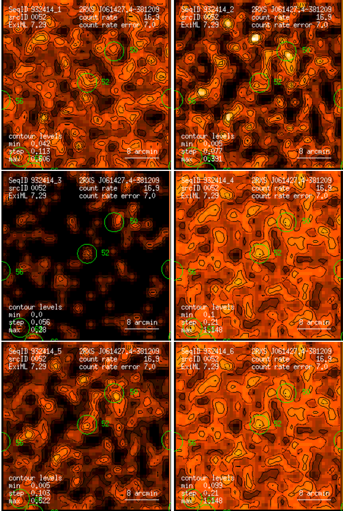
Figure 52: RASS 932414: detection 0052: band rate images, Gaussian filter: (1) PSPC channels 11 – 41, (2) 52 – 90, (3) 91 – 201, (4) 11 – 235, (5) 52 – 201, (6) 11 – 201. Broad band rates in counts/ks. Band rate contour levels in counts/ks/arcmin 2 .
