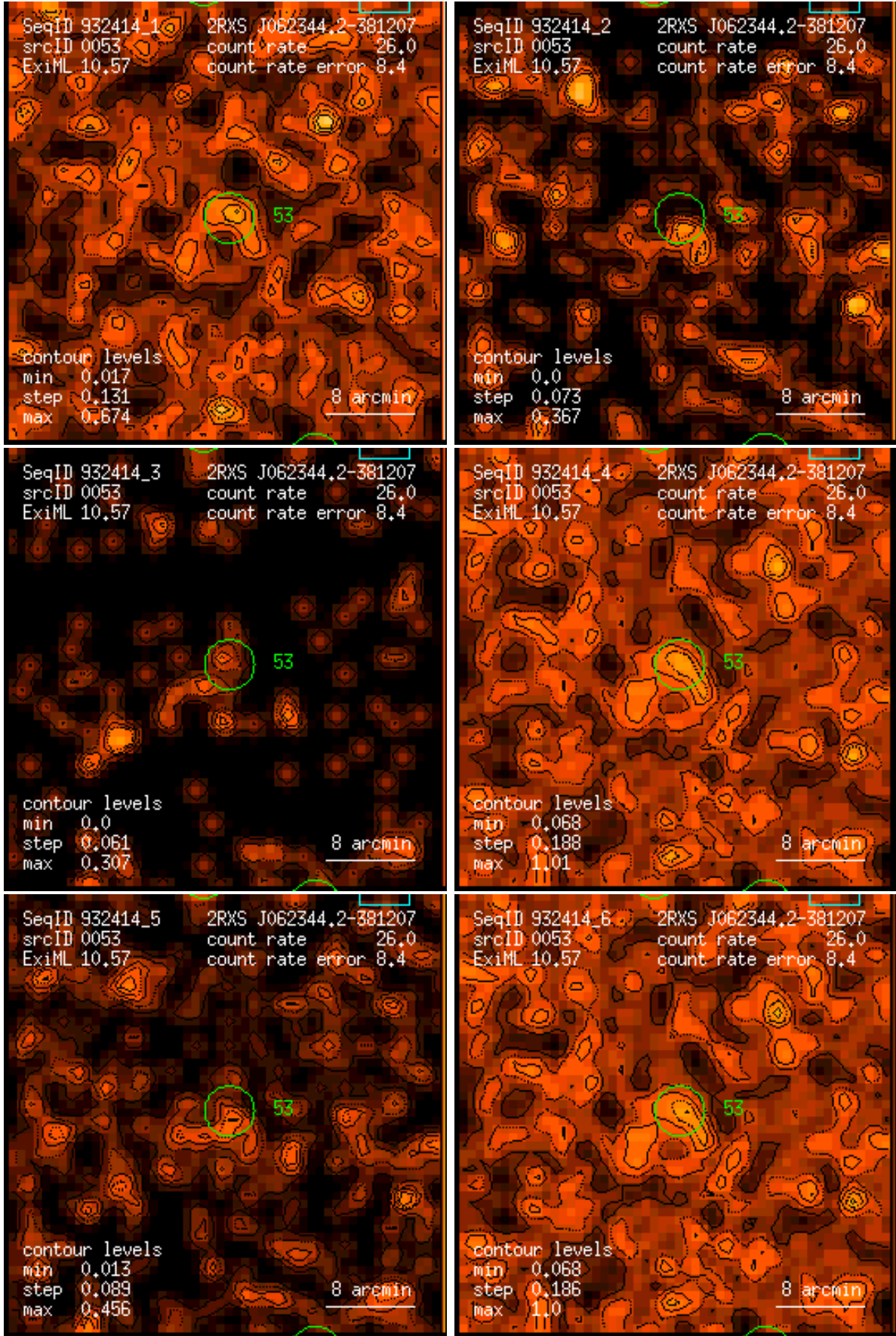
Figure 53: RASS 932414: detection 0053: band rate images, Gaussian filter: (1) PSPC channels 11 – 41, (2) 52 – 90, (3) 91 – 201, (4) 11 – 235, (5) 52 – 201, (6) 11 – 201. Broad band rates in counts/ks. Band rate contour levels in counts/ks/arcmin 2 .
