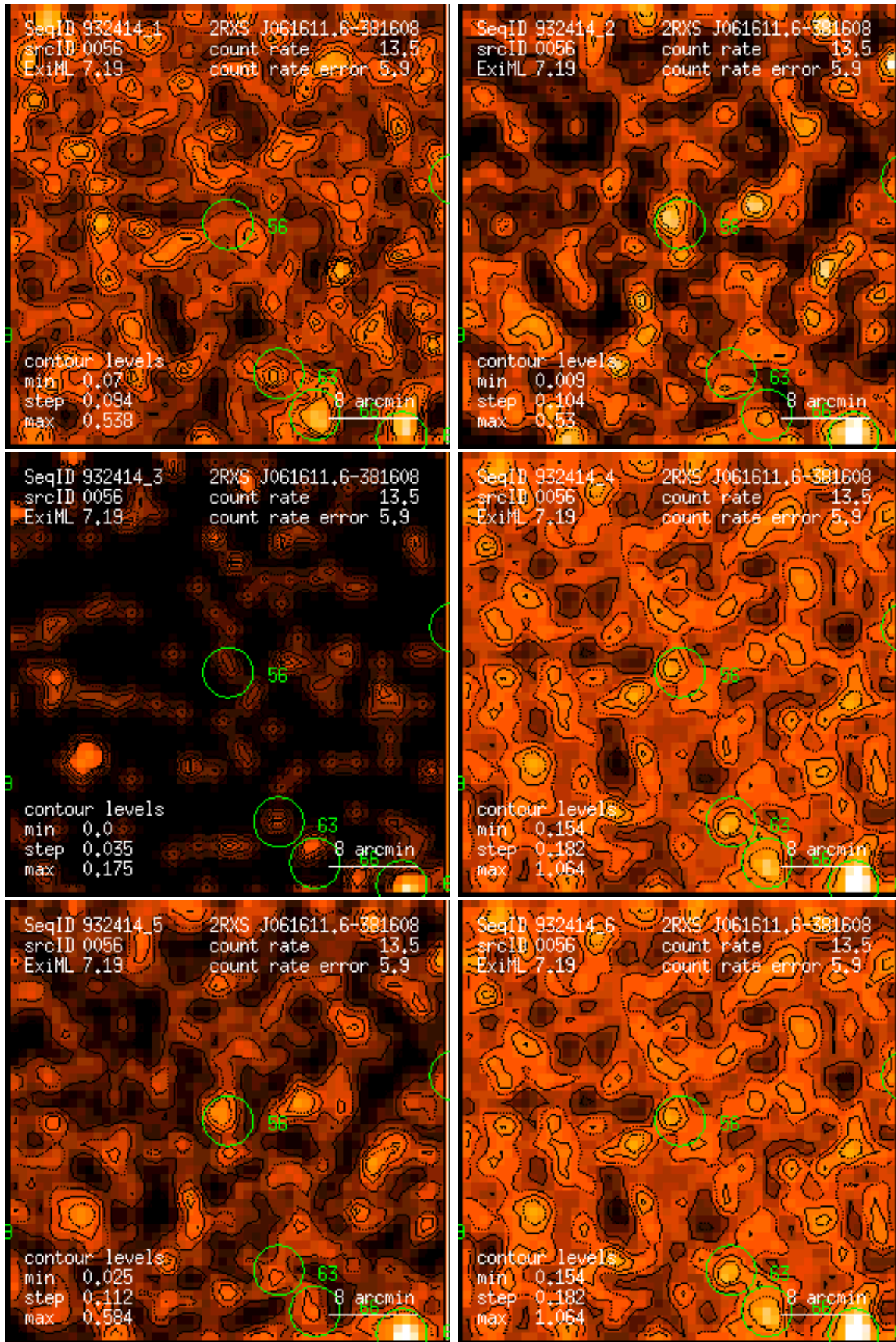
Figure 56: RASS 932414: detection 0056: band rate images, Gaussian filter: (1) PSPC channels 11 – 41, (2) 52 – 90, (3) 91 – 201, (4) 11 – 235, (5) 52 – 201, (6) 11 – 201. Broad band rates in counts/ks. Band rate contour levels in counts/ks/arcmin 2 .
