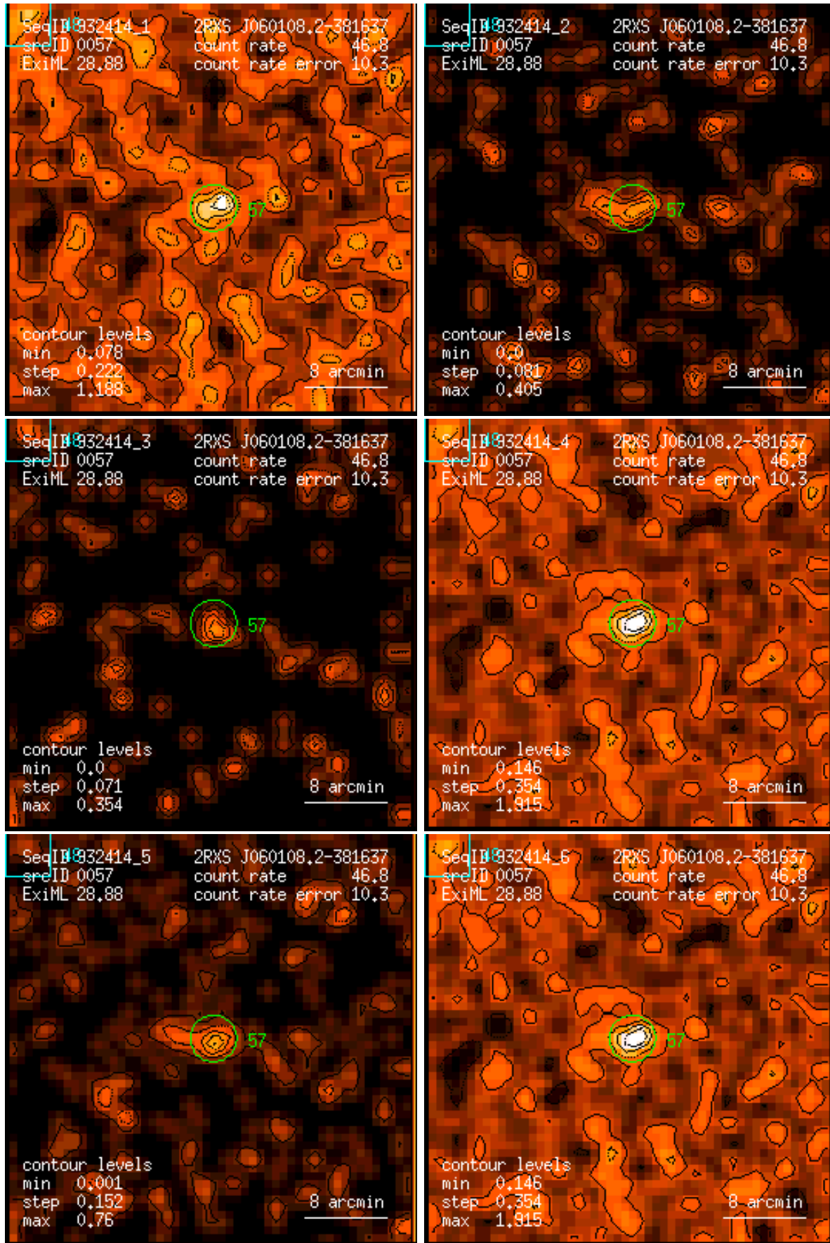
Figure 57: RASS 932414: detection 0057: band rate images, Gaussian filter: (1) PSPC channels 11 – 41, (2) 52 – 90, (3) 91 – 201, (4) 11 – 235, (5) 52 – 201, (6) 11 – 201. Broad band rates in counts/ks. Band rate contour levels in counts/ks/arcmin 2 .
