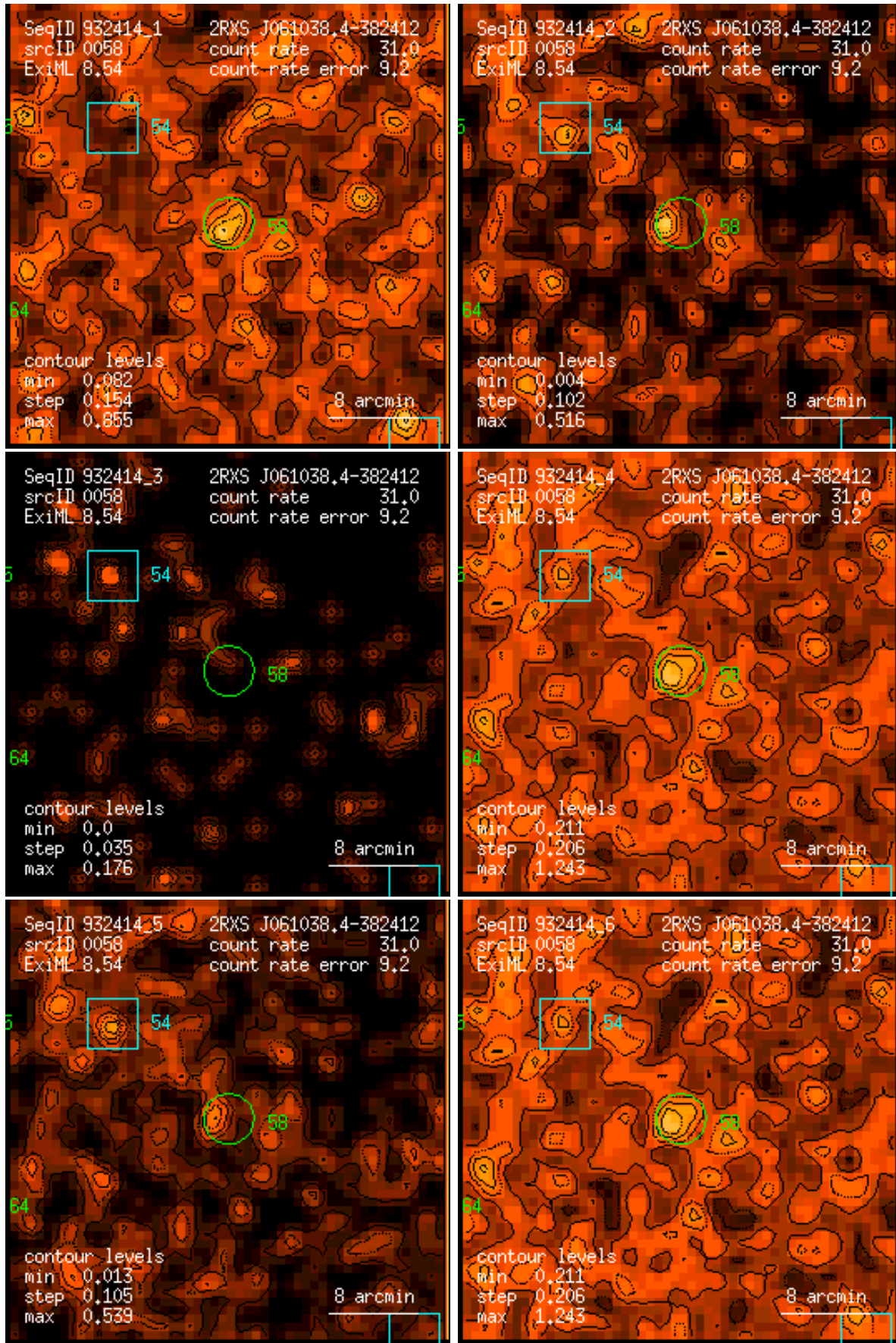
Figure 58: RASS 932414: detection 0058: band rate images, Gaussian filter: (1) PSPC channels 11 – 41, (2) 52 – 90, (3) 91 – 201, (4) 11 – 235, (5) 52 – 201, (6) 11 – 201. Broad band rates in counts/ks. Band rate contour levels in counts/ks/arcmin 2 .
