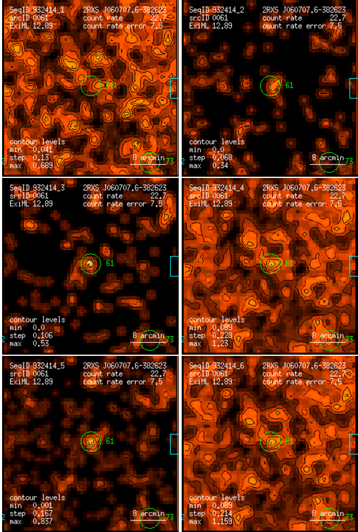
Figure 61: RASS 932414: detection 0061: band rate images, Gaussian filter: (1) PSPC channels 11 – 41, (2) 52 – 90, (3) 91 – 201, (4) 11 – 235, (5) 52 – 201, (6) 11 – 201. Broad band rates in counts/ks. Band rate contour levels in counts/ks/arcmin 2 .
