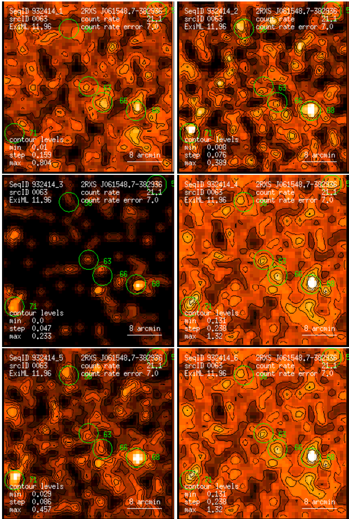
Figure 63: RASS 932414: detection 0063: band rate images, Gaussian filter: (1) PSPC channels 11 – 41, (2) 52 – 90, (3) 91 – 201, (4) 11 – 235, (5) 52 – 201, (6) 11 – 201. Broad band rates in counts/ks. Band rate contour levels in counts/ks/arcmin 2 .
