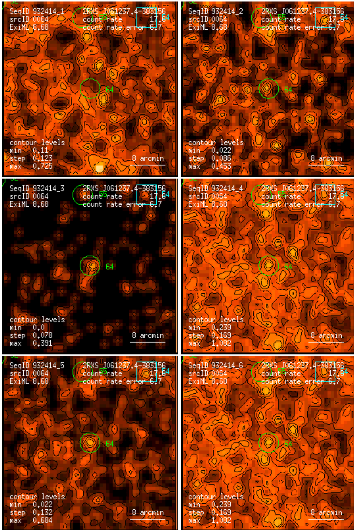
Figure 64: RASS 932414: detection 0064: band rate images, Gaussian filter: (1) PSPC channels 11 – 41, (2) 52 – 90, (3) 91 – 201, (4) 11 – 235, (5) 52 – 201, (6) 11 – 201. Broad band rates in counts/ks. Band rate contour levels in counts/ks/arcmin 2 .
