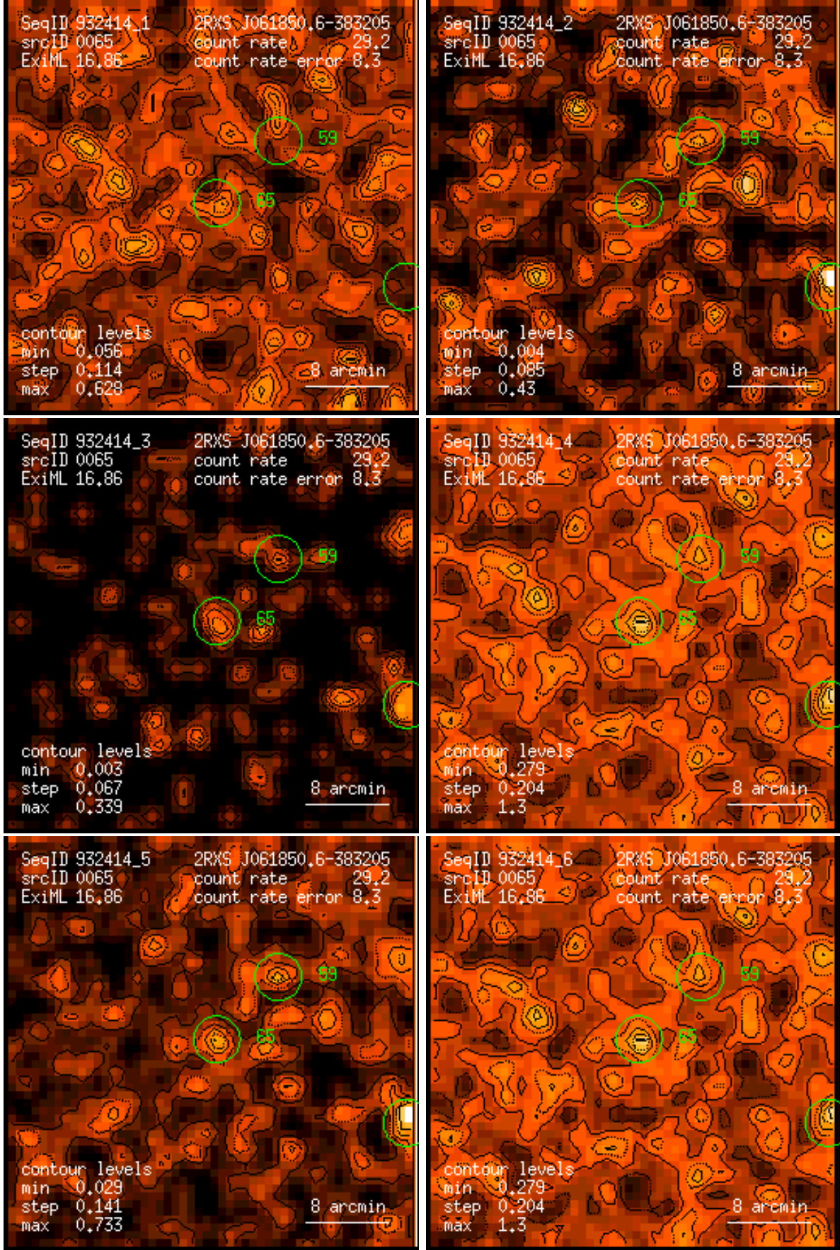
Figure 65: RASS 932414: detection 0065: band rate images, Gaussian filter: (1) PSPC channels 11 – 41, (2) 52 – 90, (3) 91 – 201, (4) 11 – 235, (5) 52 – 201, (6) 11 – 201. Broad band rates in counts/ks. Band rate contour levels in counts/ks/arcmin 2 .
