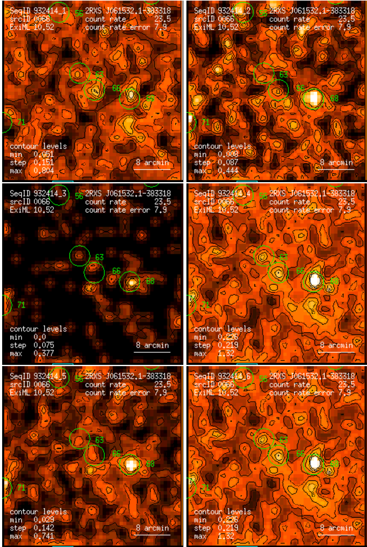
Figure 66: RASS 932414: detection 0066: band rate images, Gaussian filter: (1) PSPC channels 11 – 41, (2) 52 – 90, (3) 91 – 201, (4) 11 – 235, (5) 52 – 201, (6) 11 – 201. Broad band rates in counts/ks. Band rate contour levels in counts/ks/arcmin 2 .
