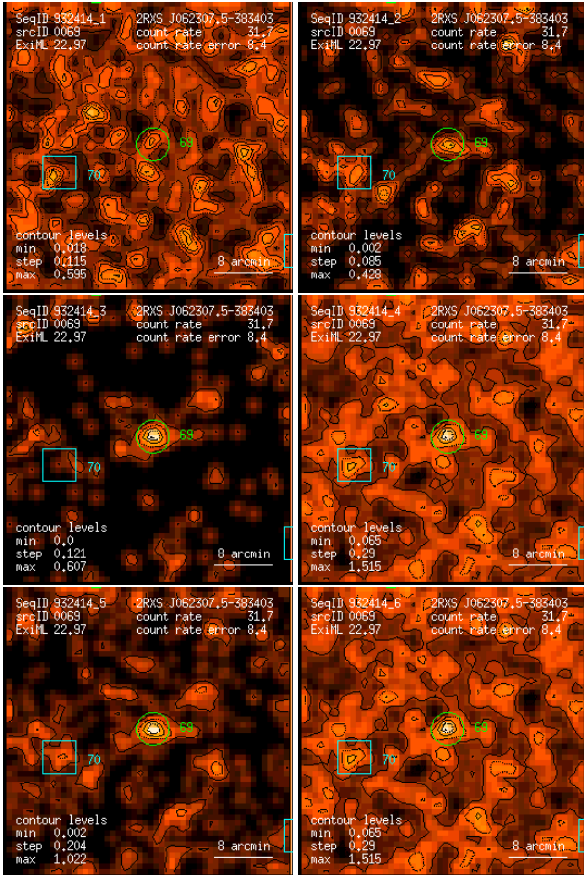
Figure 69: RASS 932414: detection 0069: band rate images, Gaussian filter: (1) PSPC channels 11 – 41, (2) 52 – 90, (3) 91 – 201, (4) 11 – 235, (5) 52 – 201, (6) 11 – 201. Broad band rates in counts/ks. Band rate contour levels in counts/ks/arcmin 2 .
